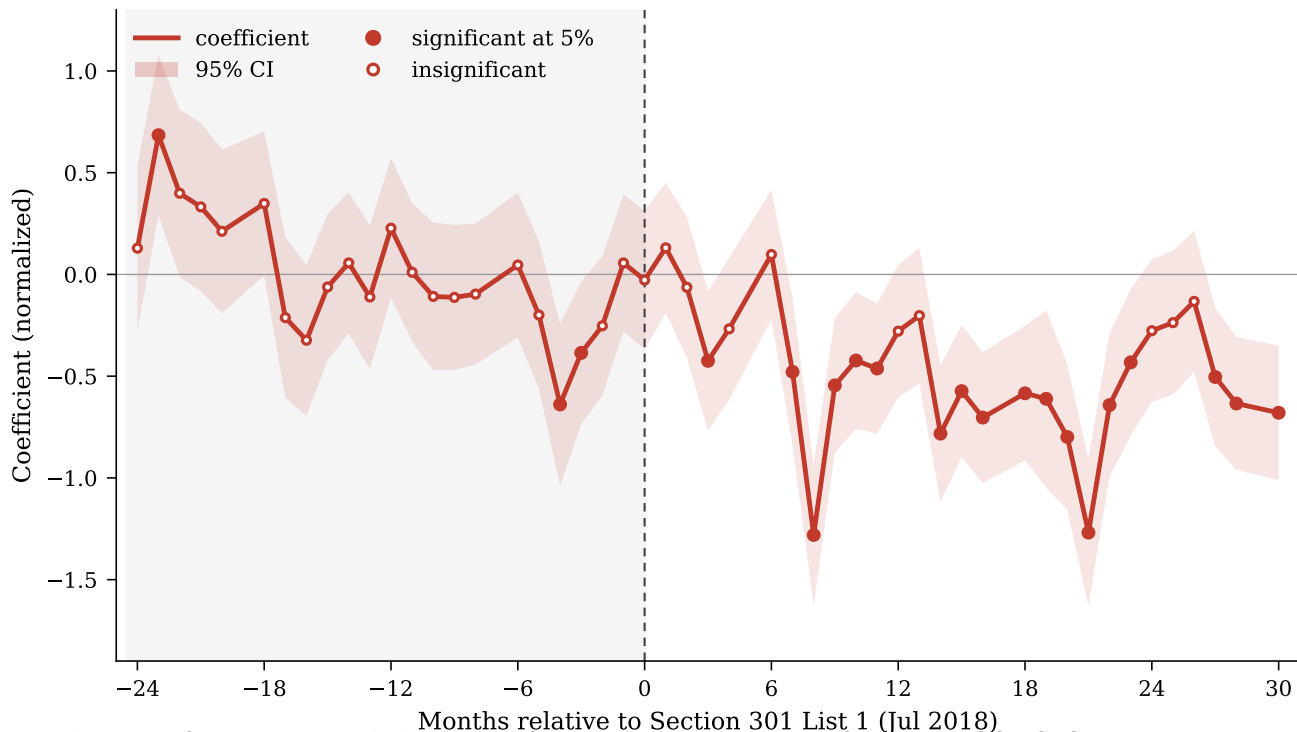
Figure 4. Event study --- CHN → MEX manufacturing exports (deflection test)
