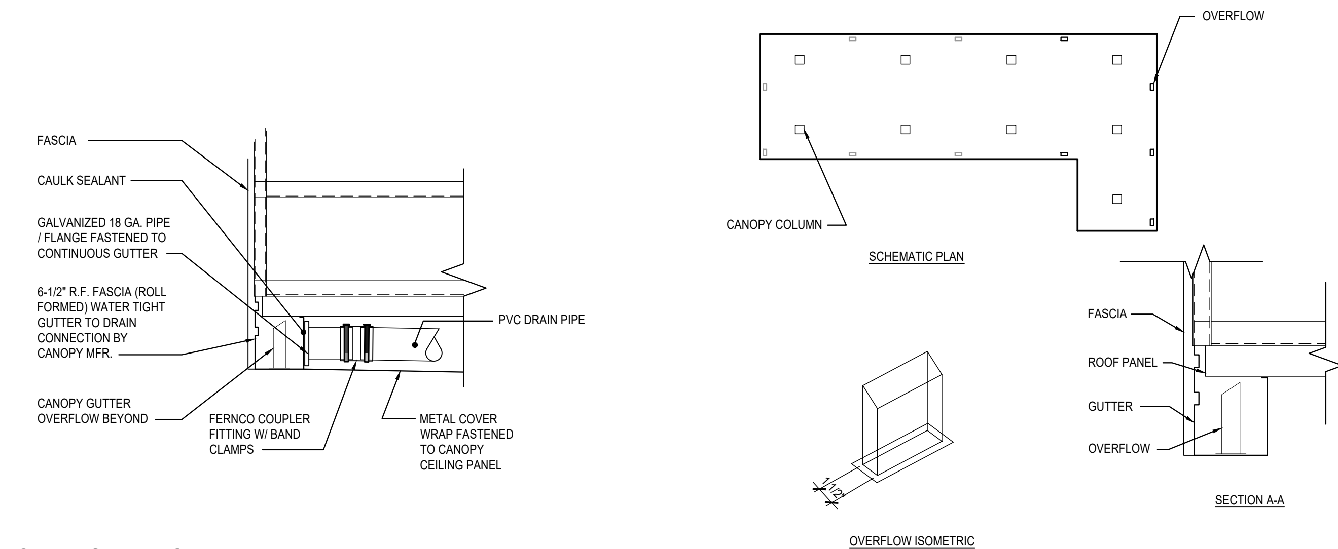
16 CANOPY GUTTER AT DRAIN CONNECTION
