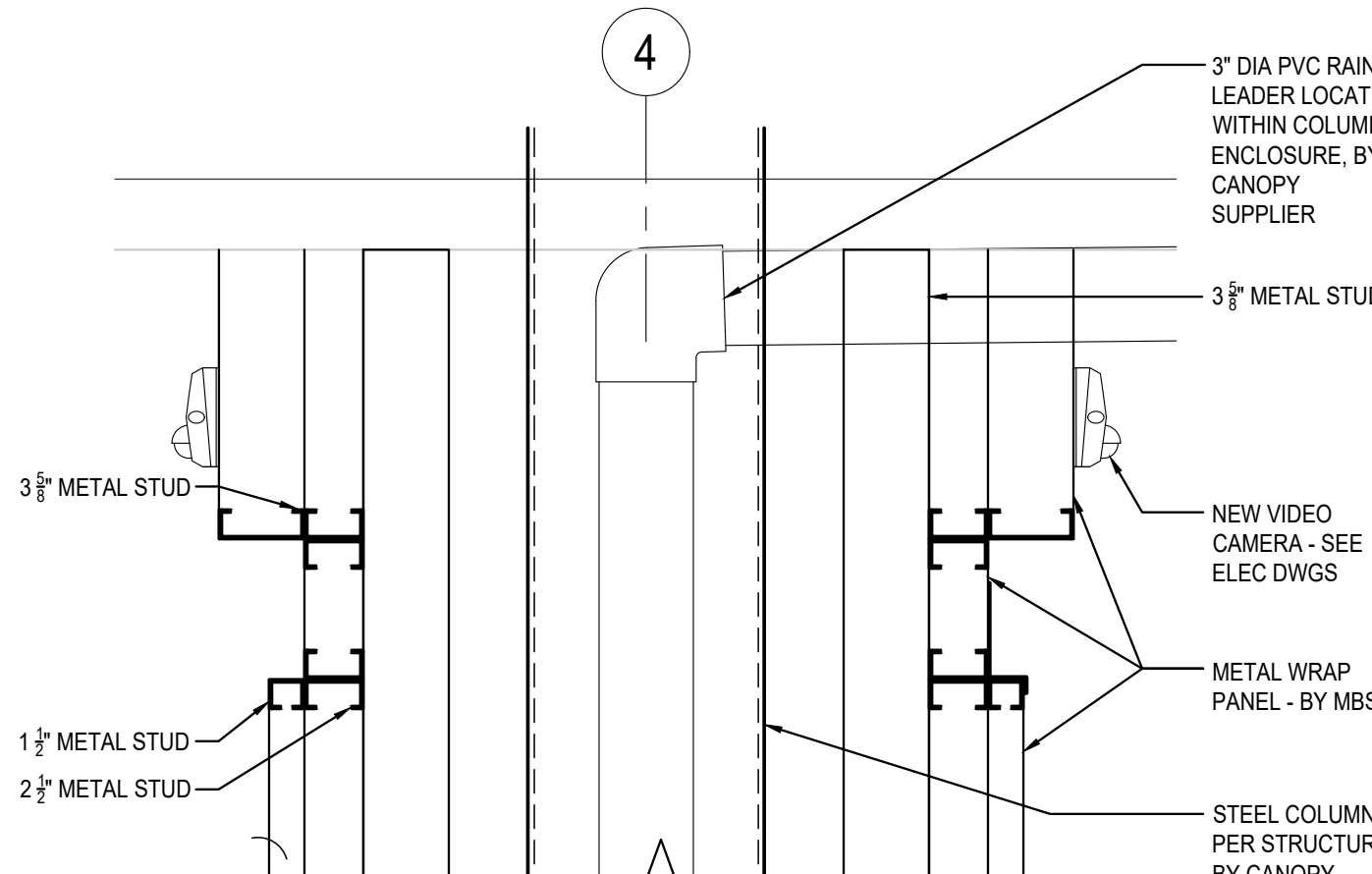
13 METAL TO METAL DETAIL
