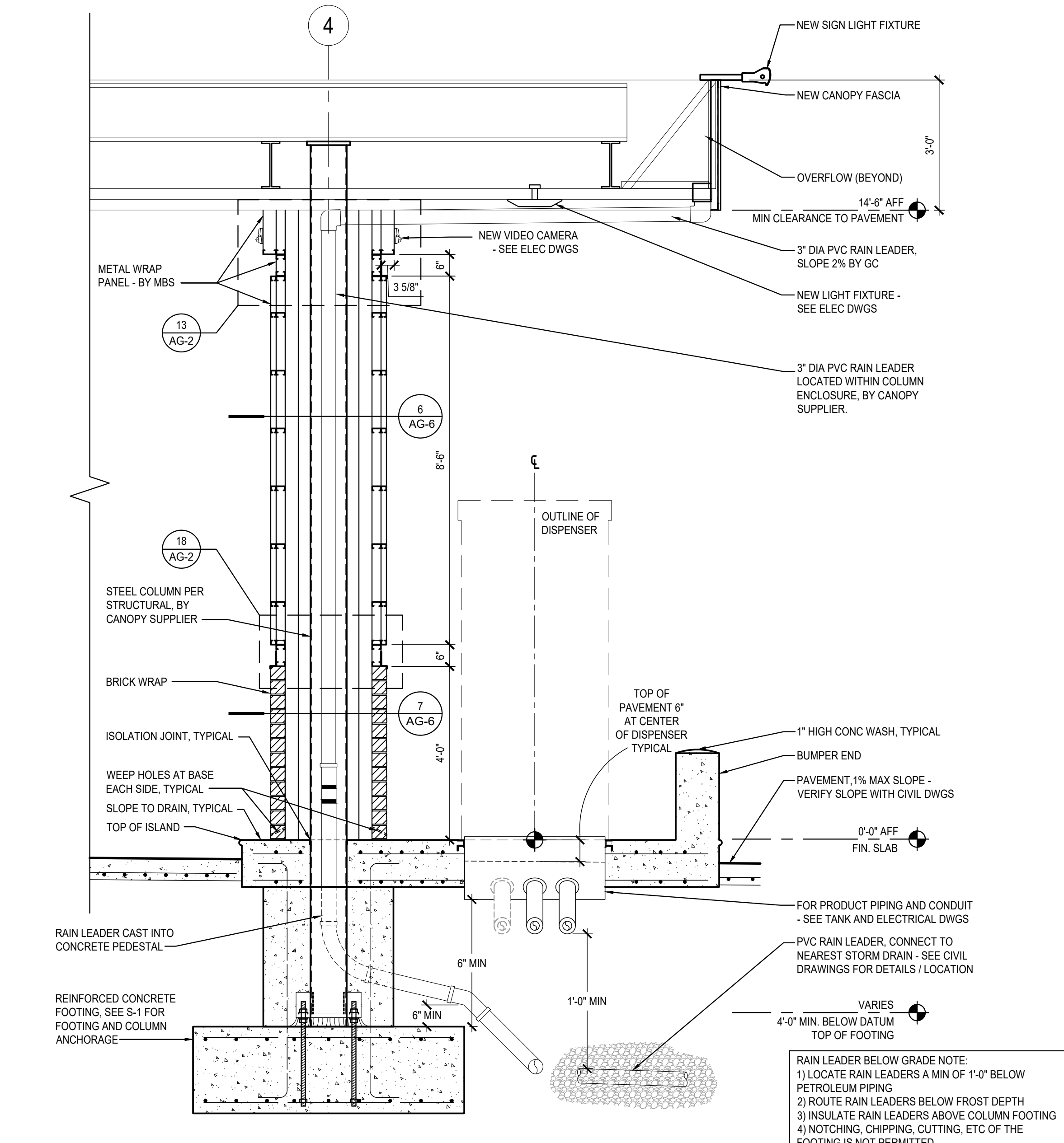
19 CANOPY FASCIA / COLUMN SECTION
