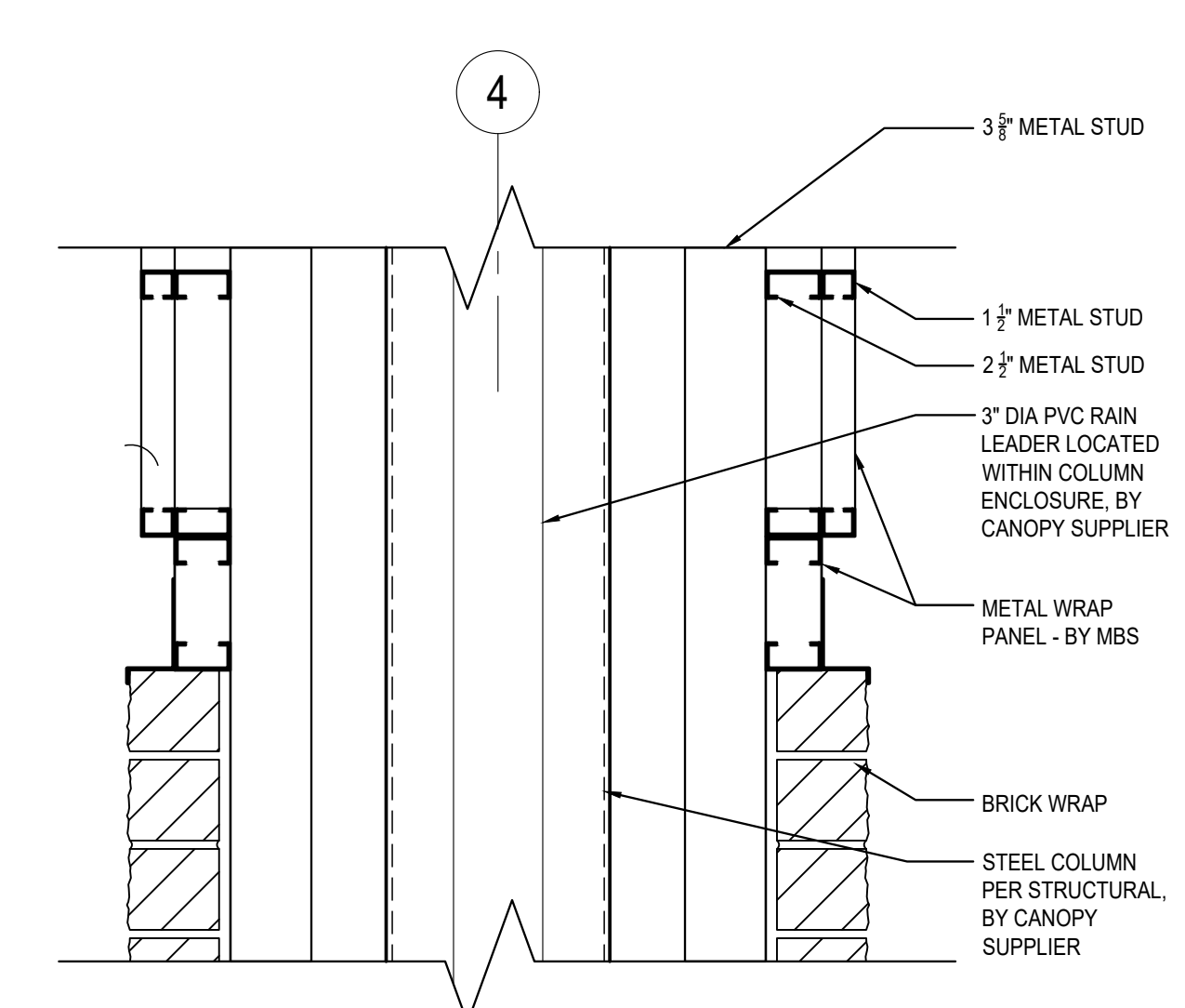
18 BRICK TO METAL DETAIL
