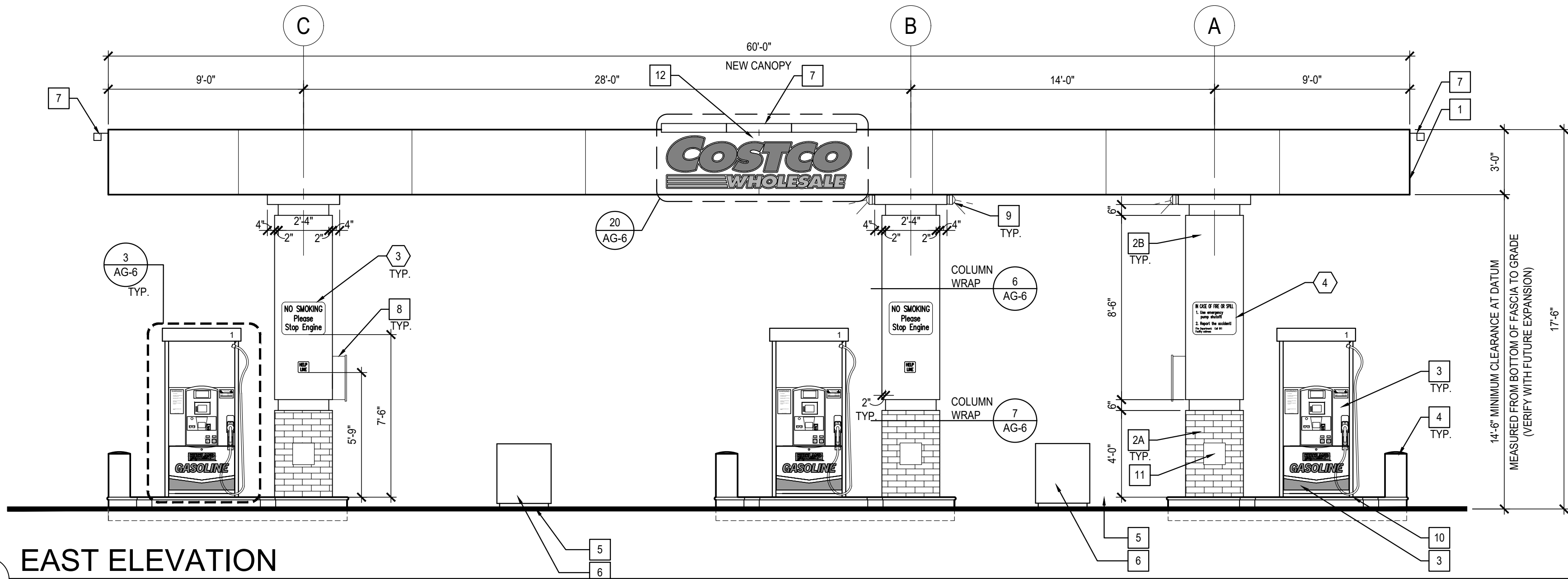
6 EAST ELEVATION
