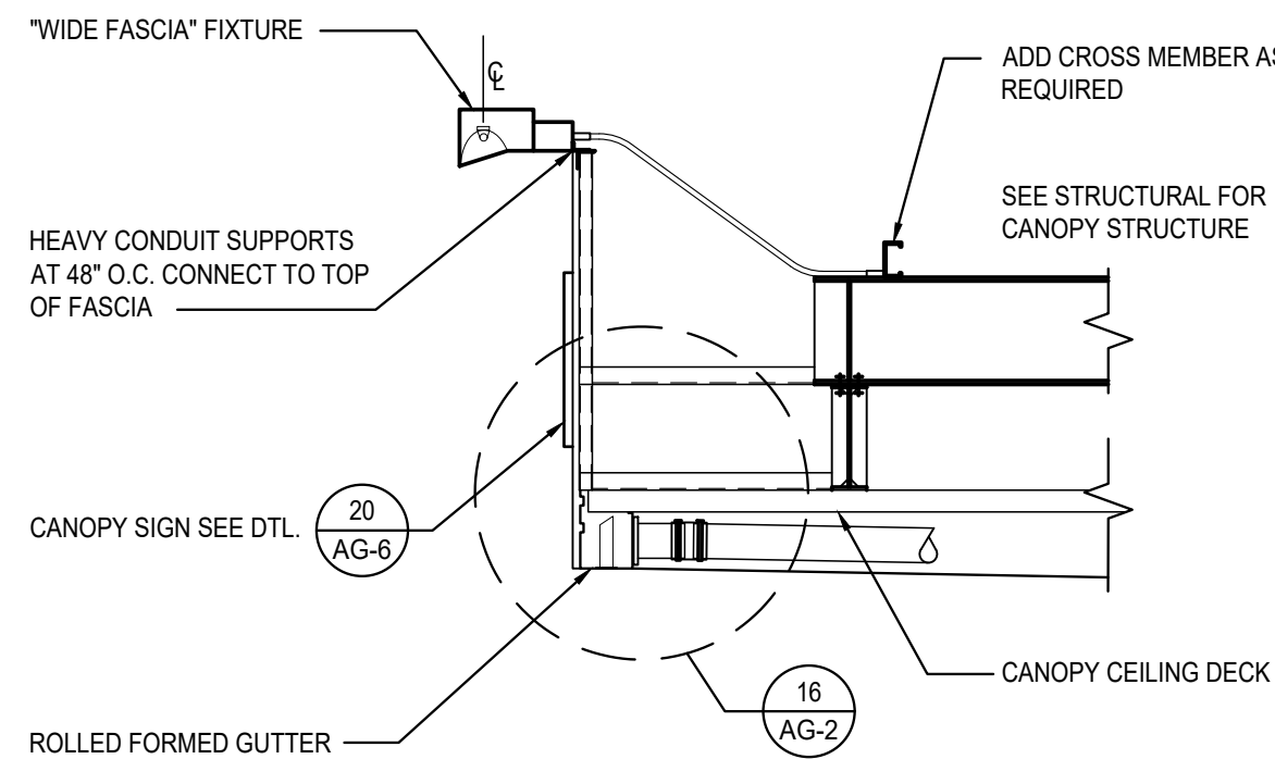
11 CANOPY FASCIA LIGHTING
