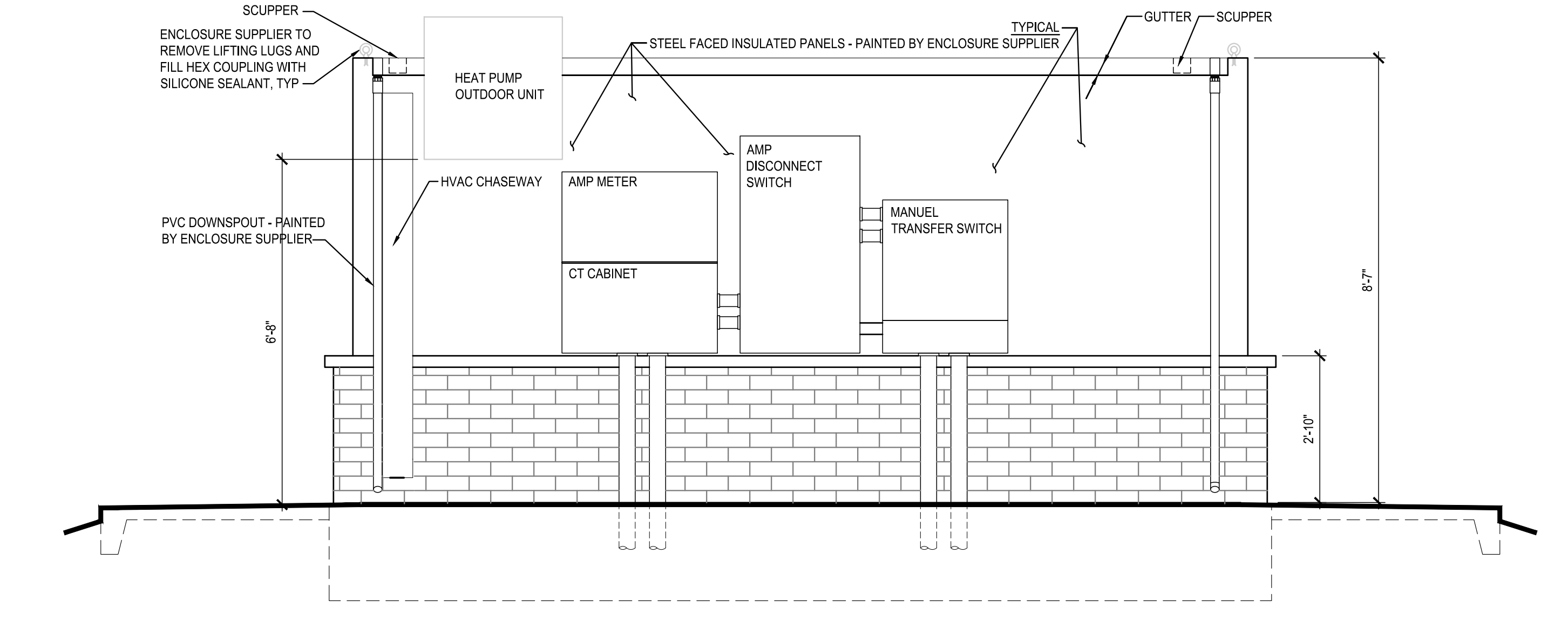
2 SIDE FACING AWAY FROM CANOPY SCALE: 1/2" = 1'-0" 1121
