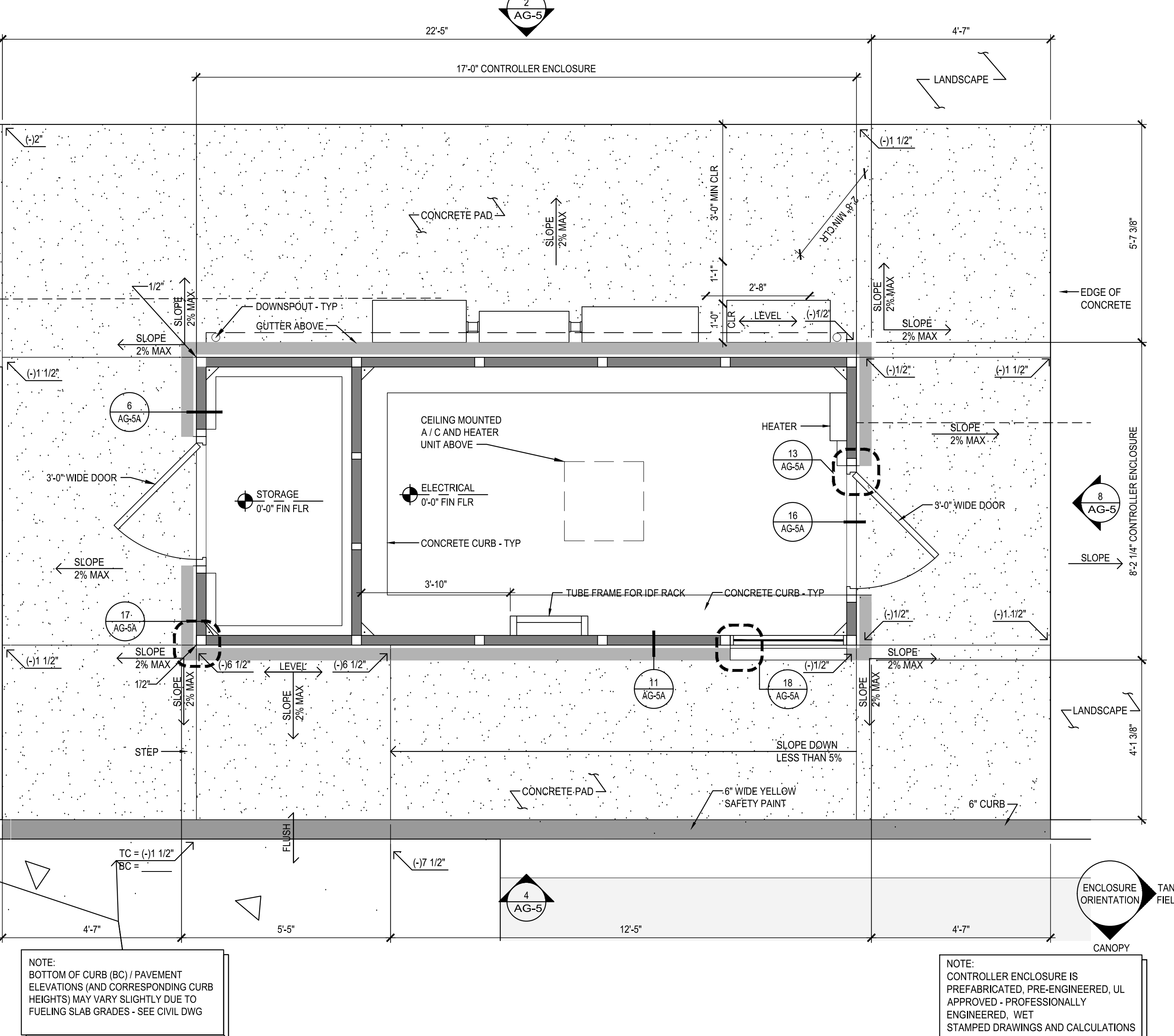
19 STANDARD CONTROLLER ENCLOSURE PLAN SCALE: 1/2" = 1'-0" 1222
