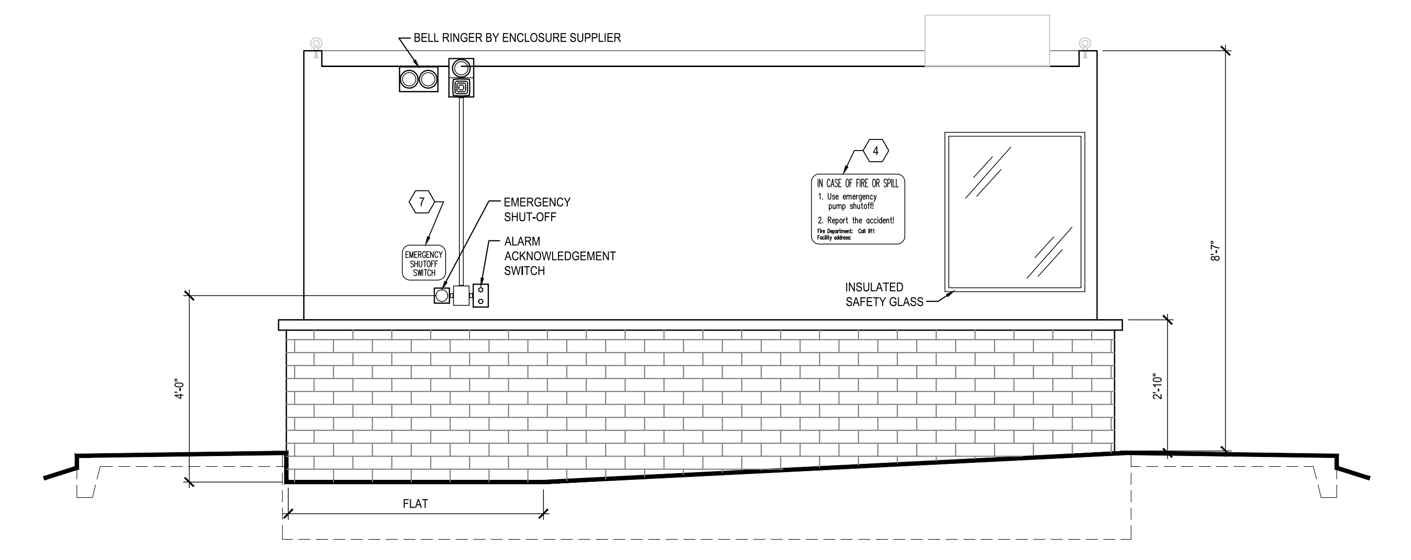
4 SIDE FACING CANOPY SCALE: 1/2" = 1'-0" 0421
