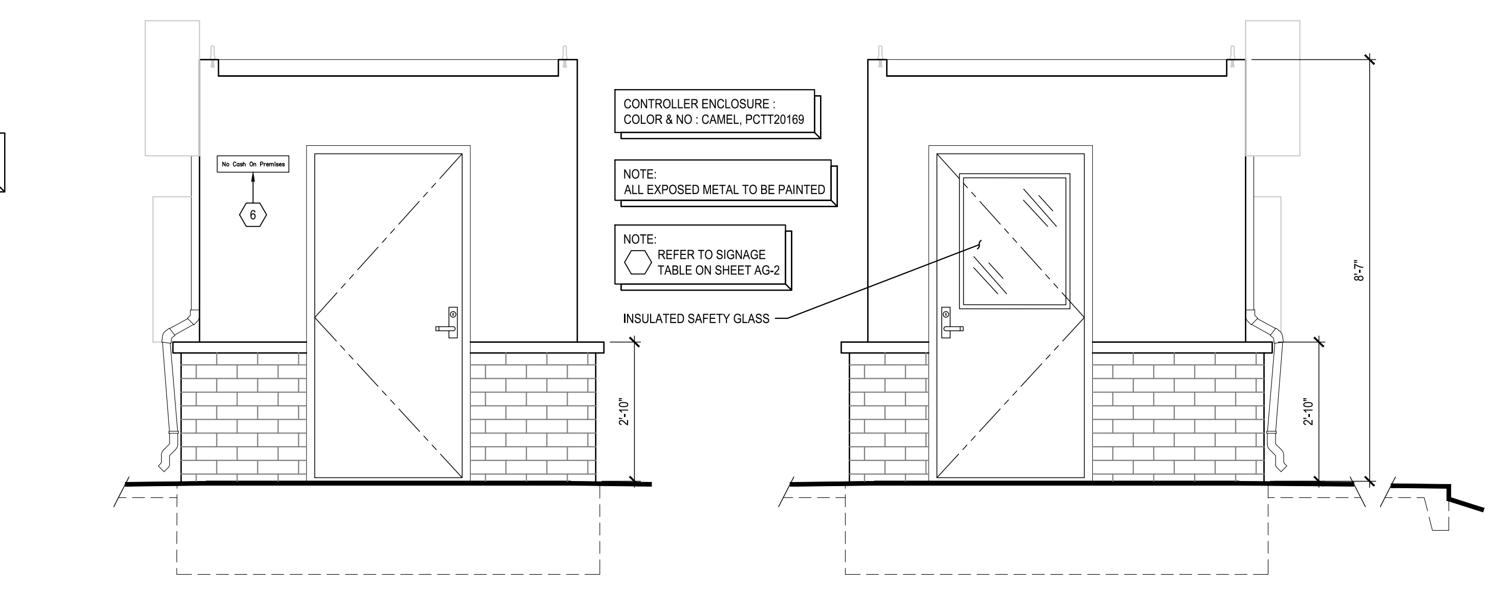
7 STORAGE ENTRY SCALE: 1/2" = 1'-0" 1222
