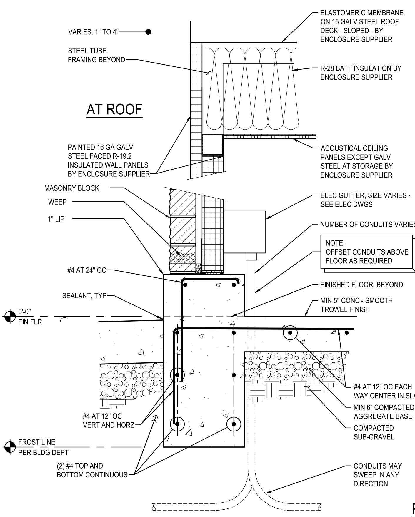
11 TYPICAL WALL SCALE: 1-1/2" = 1'-0" 0421
