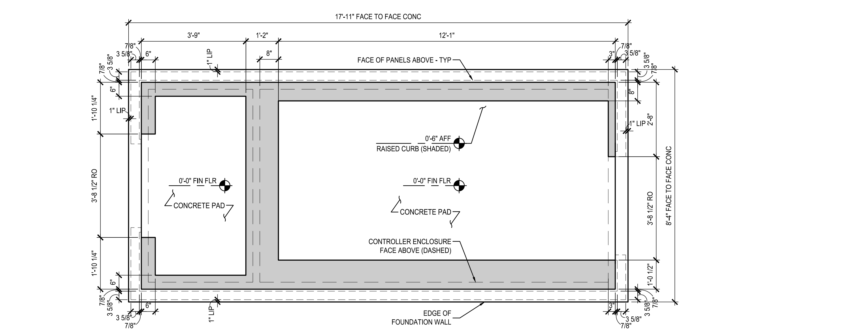
9 FOUNDATION PLAN SCALE: 1/2" = 1'-0" 1222
