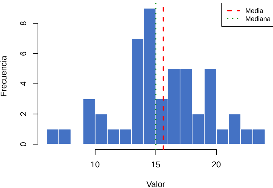
Histograma
