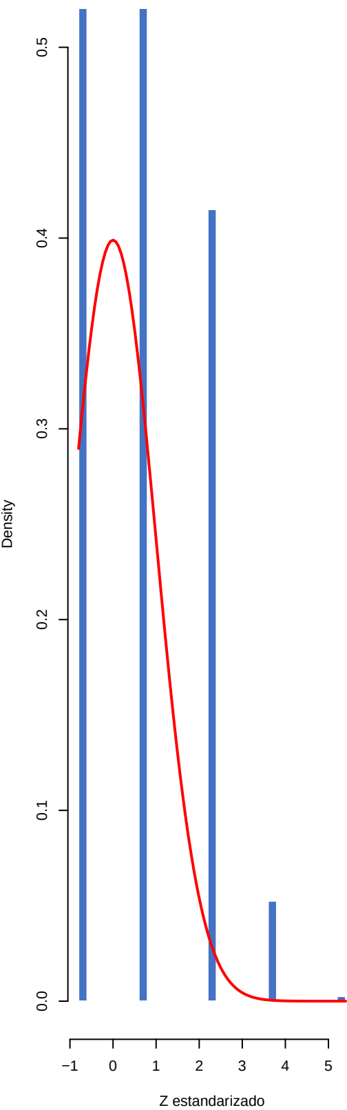
Bernoulli(0.1) n=5
