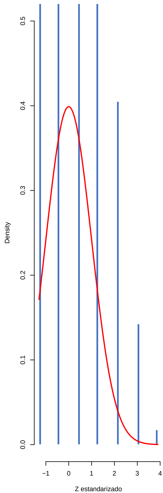
Bernoulli(0.1) n=15
