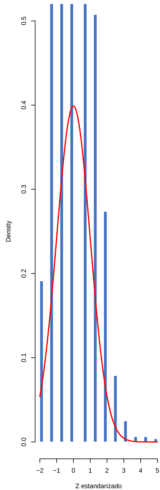
Bernoulli(0.1) n=30
