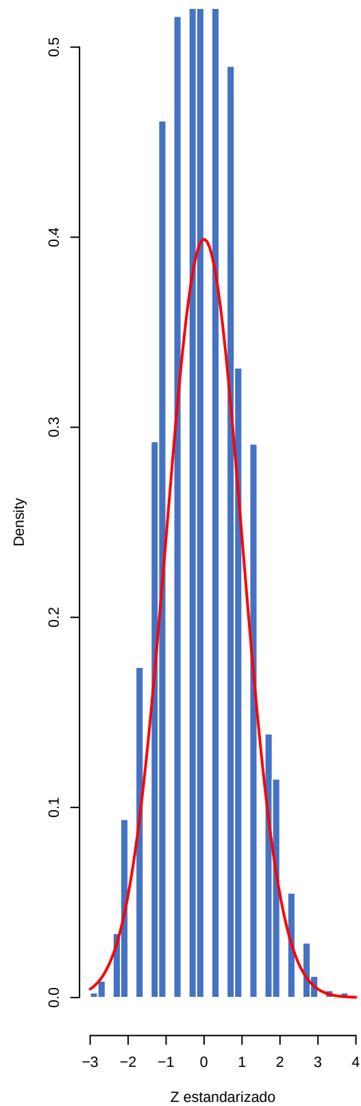
Bernoulli(0.1) n=100
