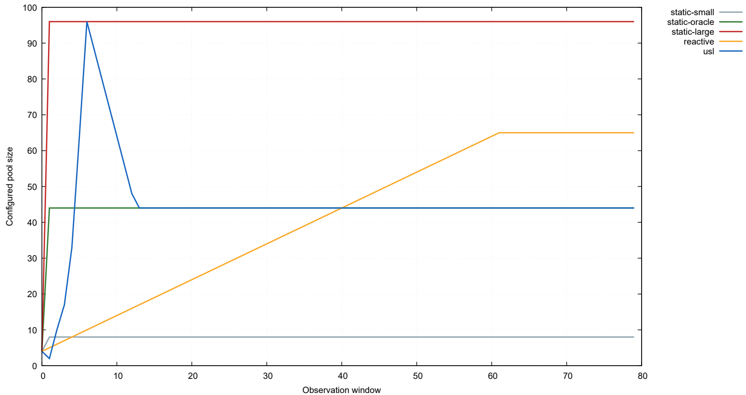
Pool size convergence per policy
