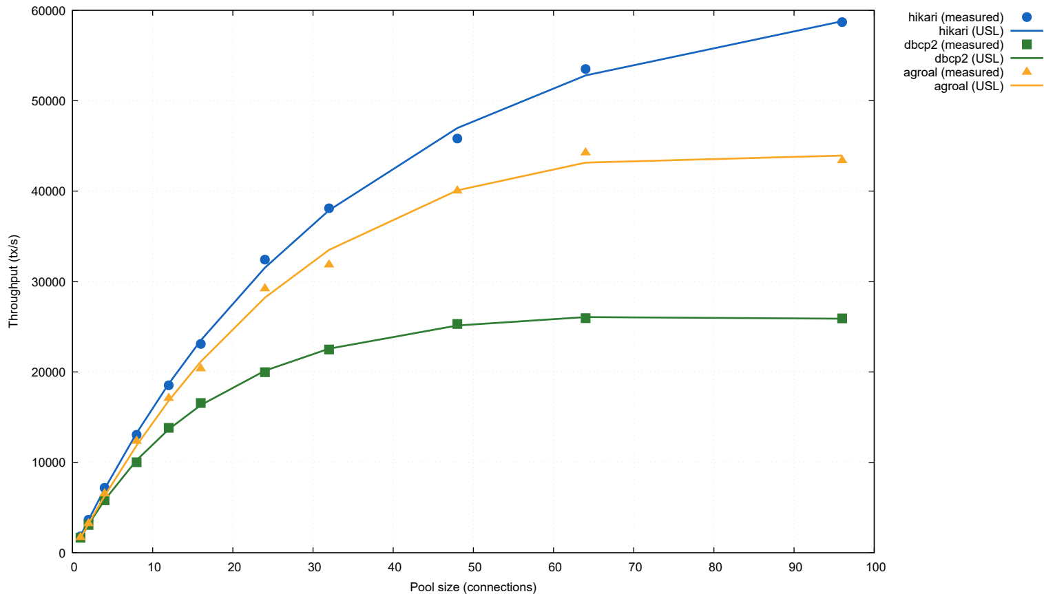
Throughput vs. pool size: measured points and fitted USL
