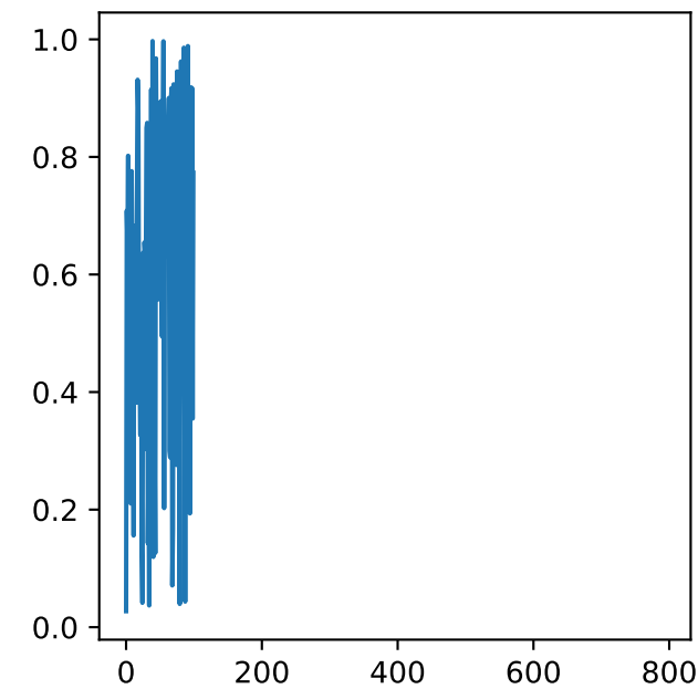
x[n]
