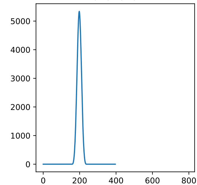
(x^2) * (x^2)
