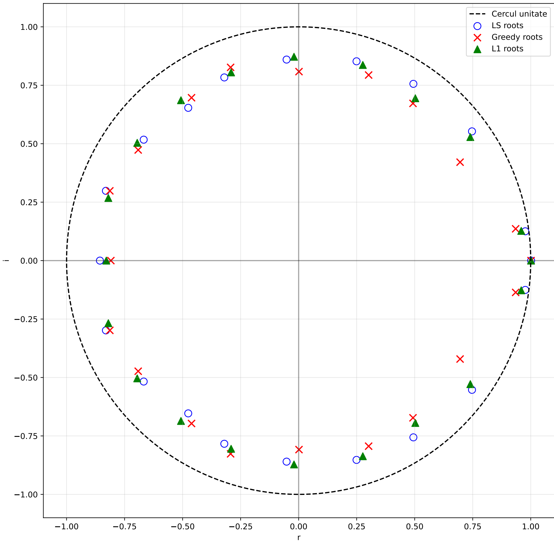
Stationaritate modele
