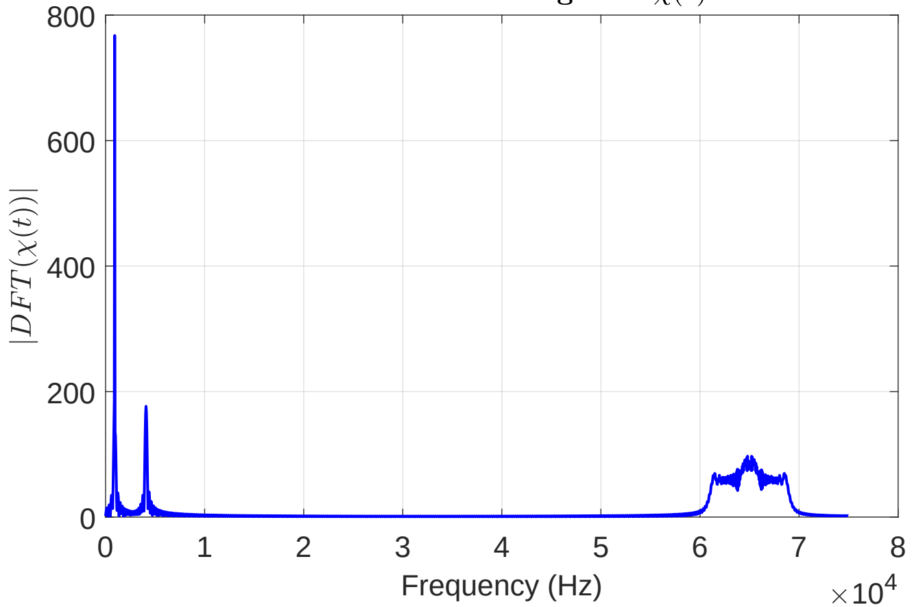
DFT of Mixed Signal – \chi(t)
