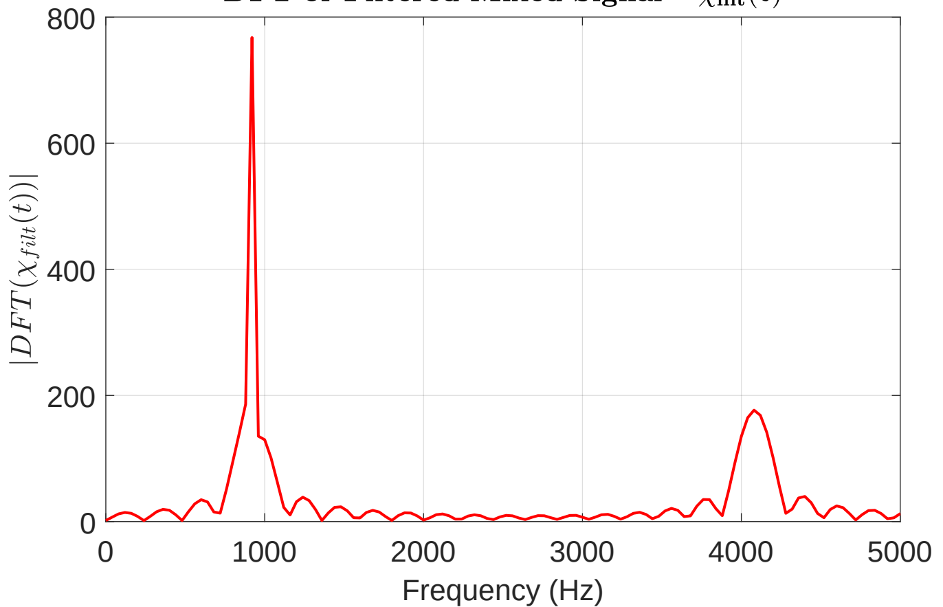
DFT of Filtered Mixed Signal – \chi_{filt}(t)
