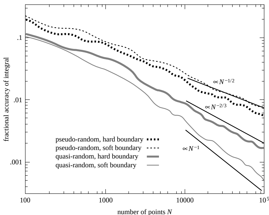
Figure 7.7.2. Fractional accuracy of Monte Carlo integrations as a function of number of points sampled, for two different integrands and two different methods of choosing random points. The quasi-random Sobol' sequence converges much more rapidly than a conventional pseudo-random sequence. Quasi-random sampling does better when the integrand is smooth ("soft boundary") than when it has step discontinuities ("hard boundary"). The curves shown are the r.m.s. average of 100 trials.
