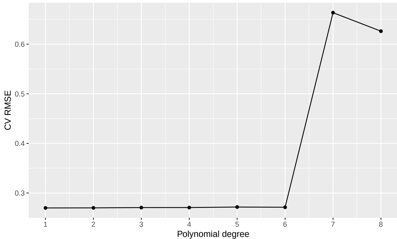
Polynomial degree tuning by 10-fold CV
