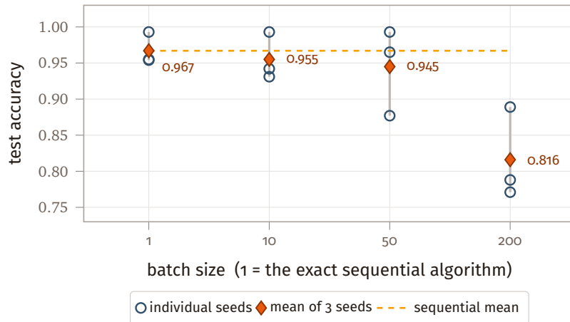
Figure 11. Noisy XOR accuracy against batch size (3 seeds). Batches up to about 50 land in the same band as the exact sequential algorithm; 200 degrades clearly. Seed-to-seed spread is wide on this task — which is itself the reason to read the individual points rather than only the means.
