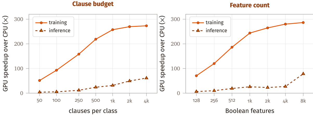
Figure 8. The GPU advantage grows with the model. Big machines — the ones the Tsetlin machine literature actually uses for images — are exactly the ones worth moving to a GPU.
