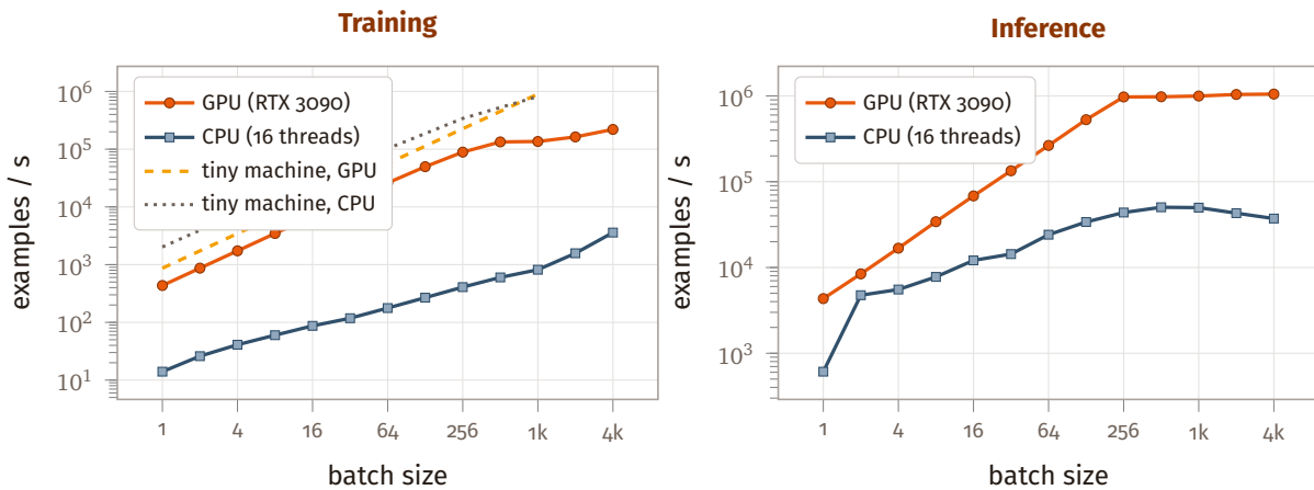
Figure 7. Throughput against batch size for a 784-feature, 500-clause-per-class machine (log-log). Training on the GPU scales almost linearly with batch size until the device saturates. The dashed line is the counter-example: a 12-feature, 10-clause machine is less work than a kernel launch, and only overtakes the CPU past batch 1024.
