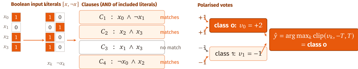
Figure 1. A Tsetlin machine classifier at inference time. Features are expanded into literals [x, \neg x] ; each clause is a conjunction of the literals its automata have decided to include ; matching clauses cast signed votes; the argmax over clipped vote sums is the prediction.
