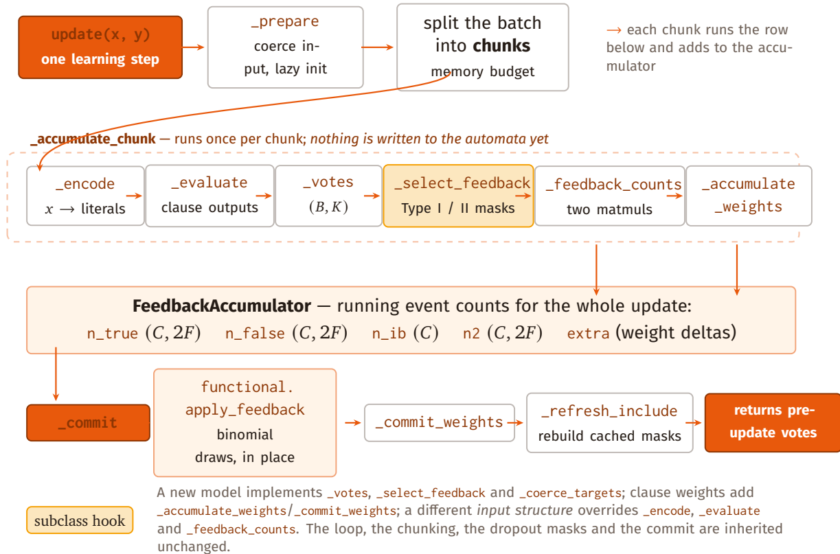
Figure 3. The update() pipeline. The batch is split into chunks that respect a memory budget; each chunk contributes event counts to a shared accumulator; the automata are written once, at the commit. Amber marks the hook a new model must implement.
