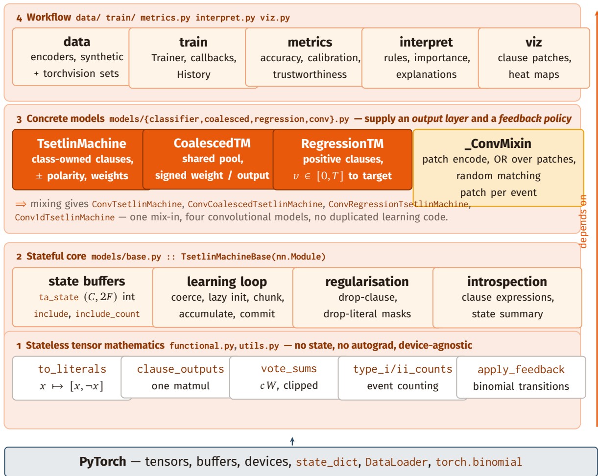
Figure 2. The four layers. Dependencies point downwards only: the learning mathematics does not know what a model is, and a model does not know what a trainer is.
