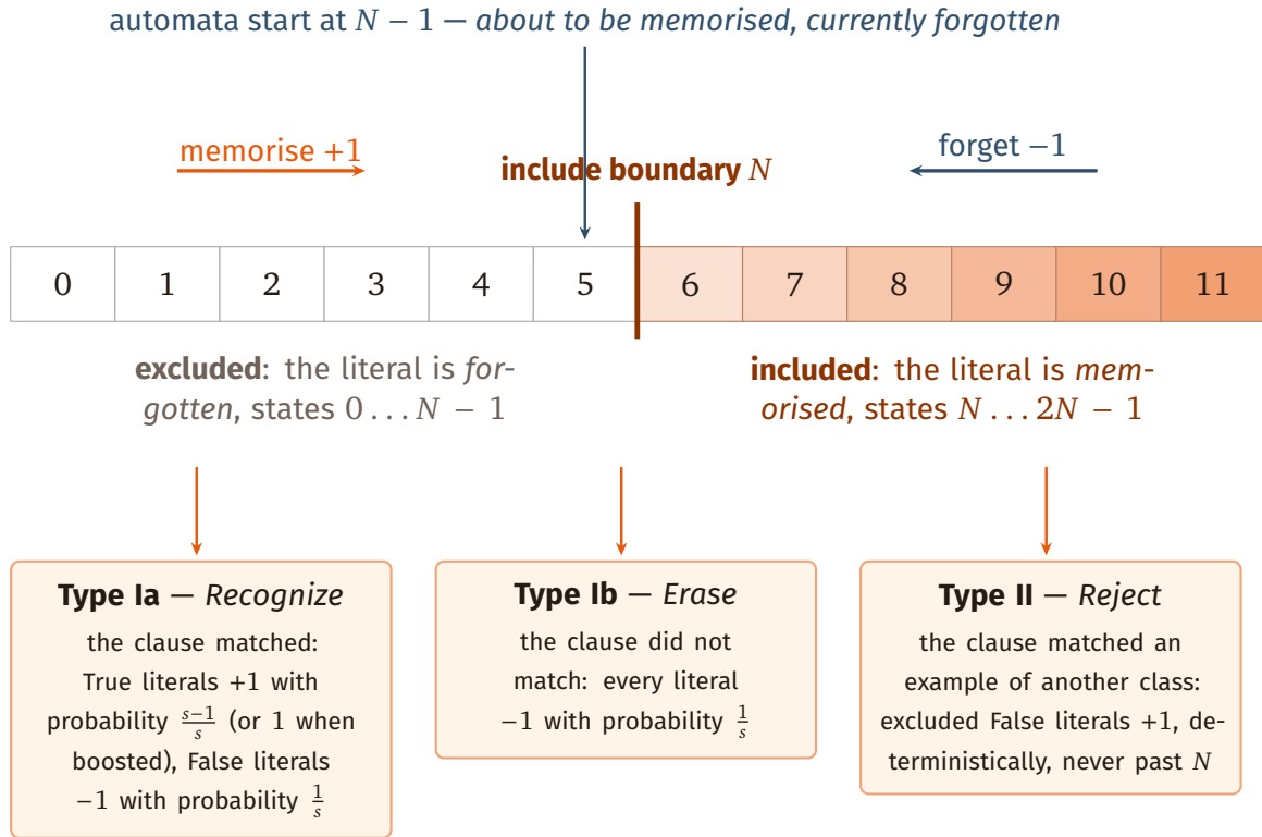
Figure 4. One Tsetlin automaton. The state line is split at N : below it the literal is forgotten, at or above it the literal is included in the clause. Deep states are hard to dislodge, states near the boundary flip easily — this is the memory that makes the machine robust to noisy examples.
