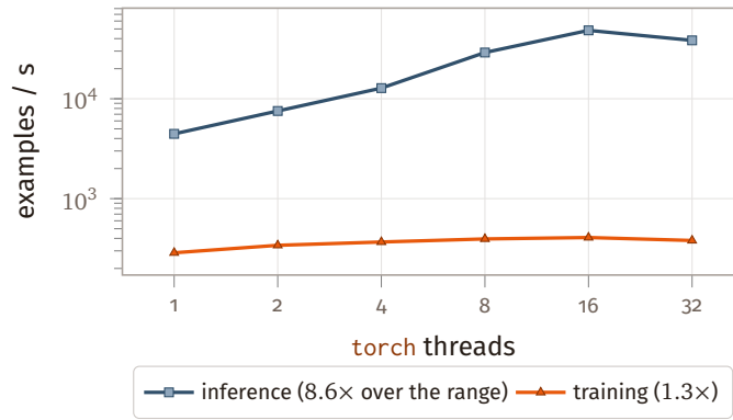
Figure 10. CPU thread scaling (5000 clauses, 784 features, batch 256).
