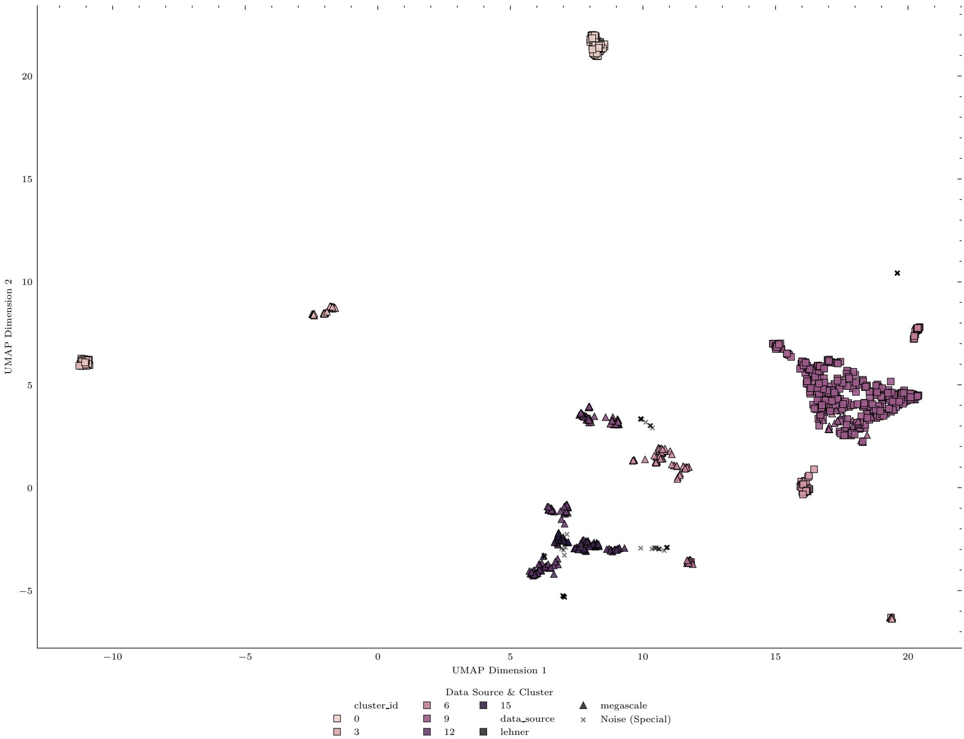
WT Protein Space with Lehner and MegaScale Data Overlays
