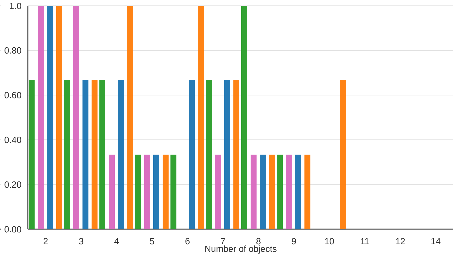
Arithmetic
