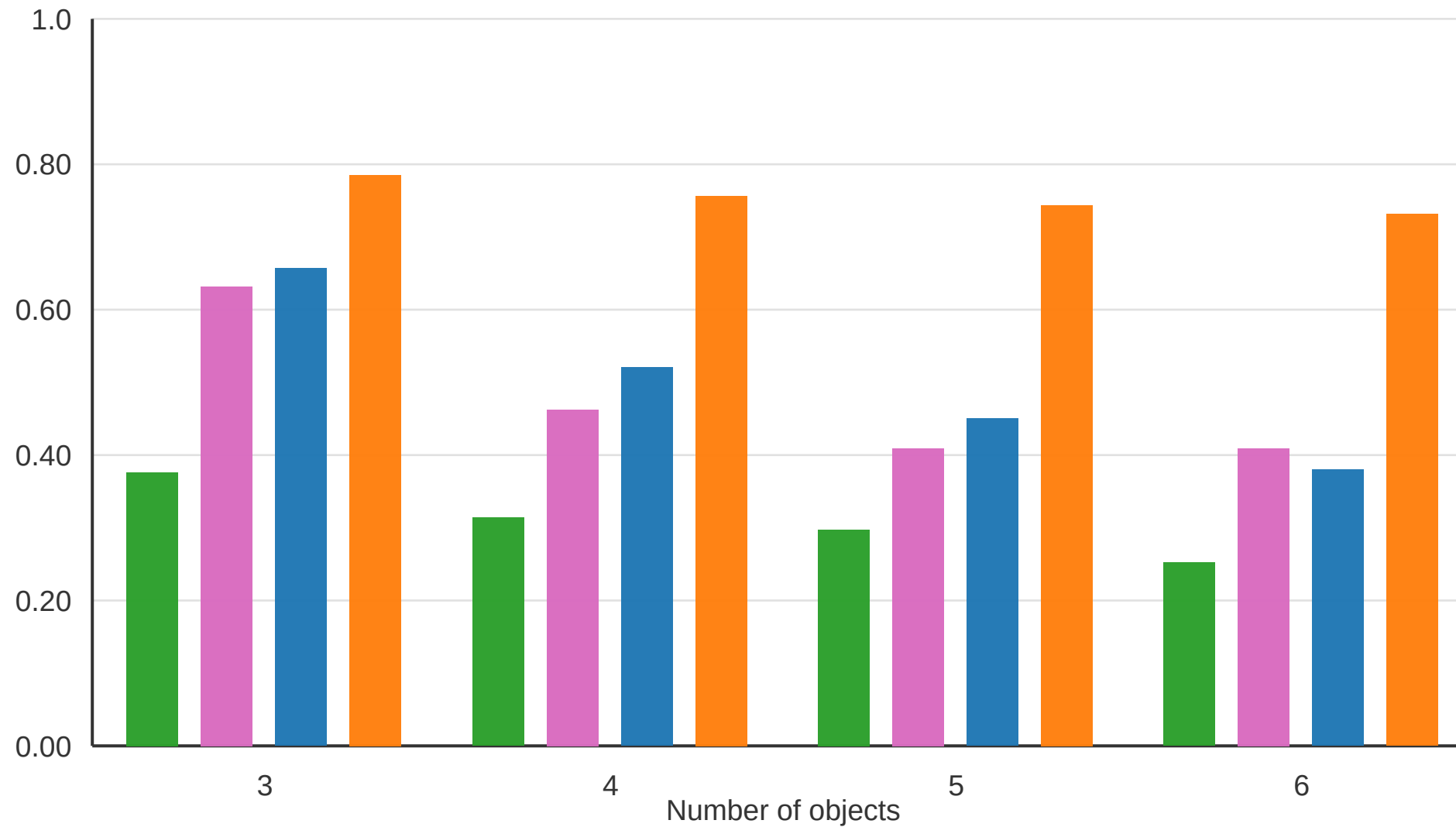
Spatial
