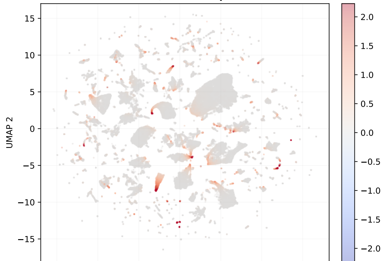
wB97X-V on BFDExt train (n=139,984 atom pairs)
