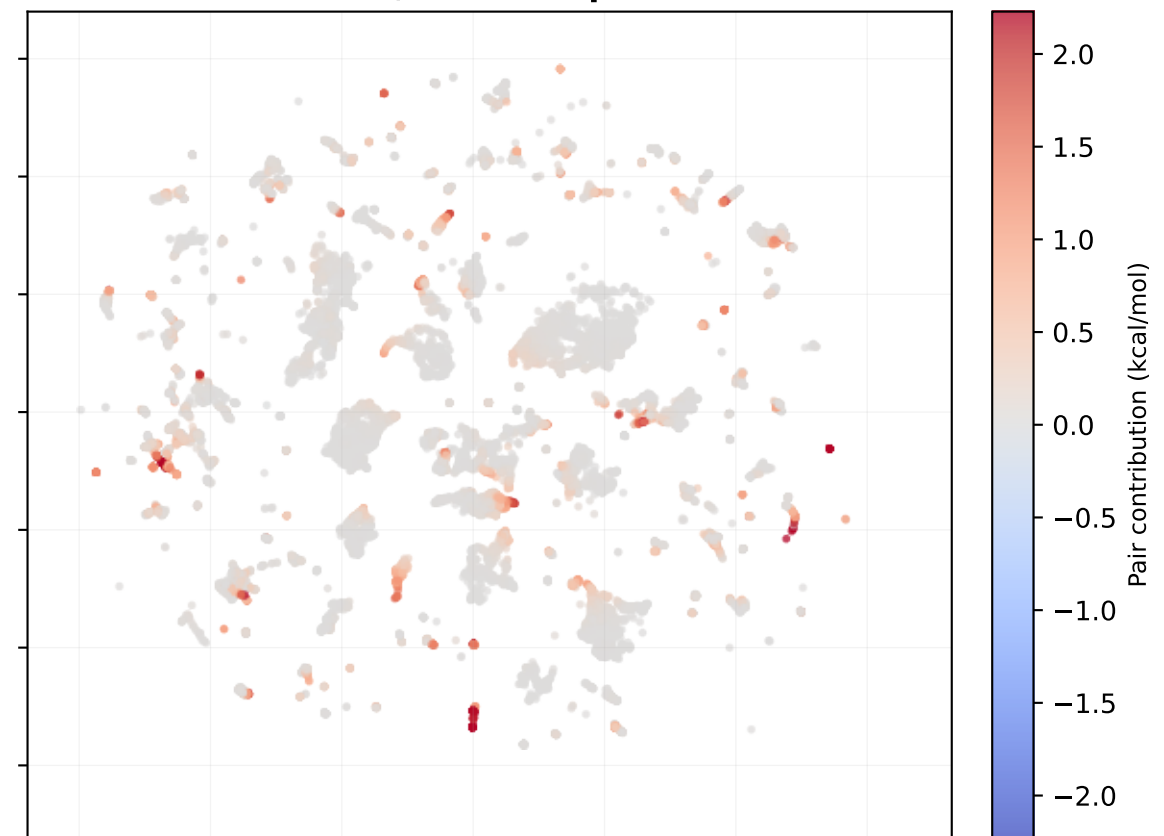
wB97X-V on HB375 (n=26,952 atom pairs)
