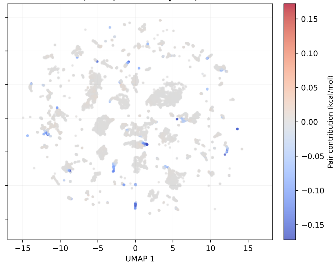
wB97X-V on HB375 (n=26,952 atom pairs)
