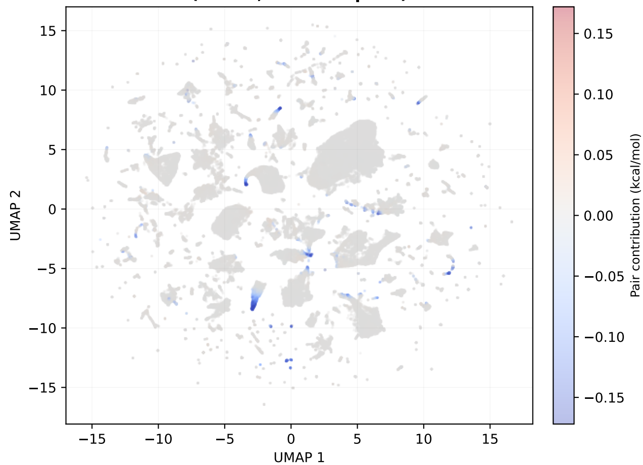
wB97X-V on BFDExt train (n=139,984 atom pairs)
