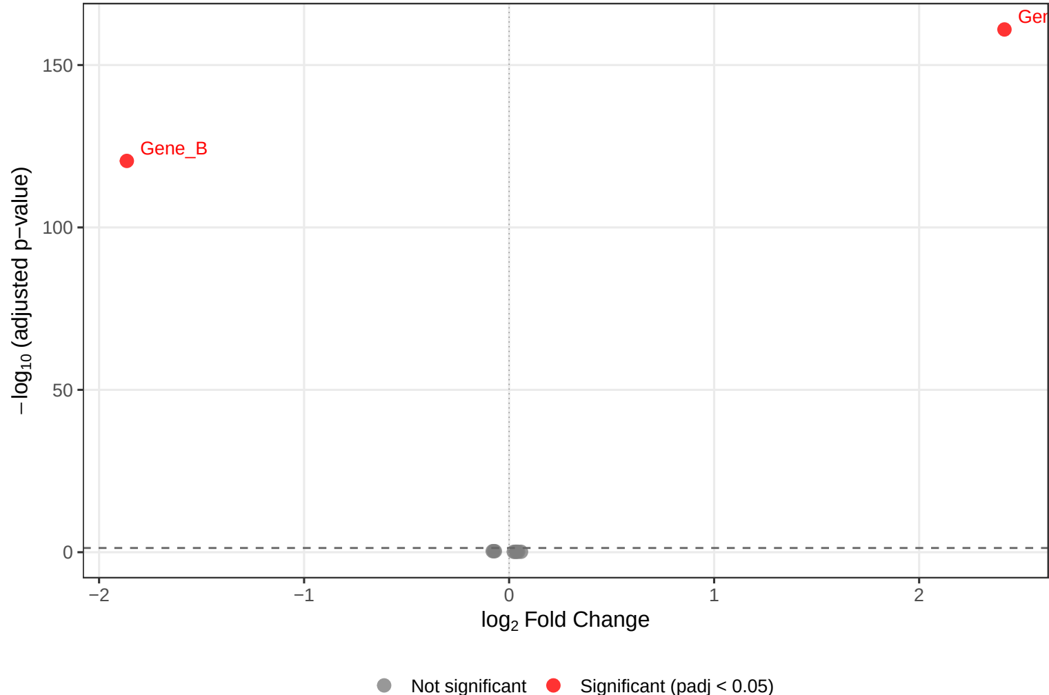
Figure 1: Volcano Plot of Differential Expression
