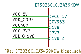
File: ET3036C_CJ3439KDW.kicad_sch
