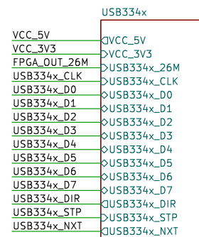
File: USB334x.kicad_sch
