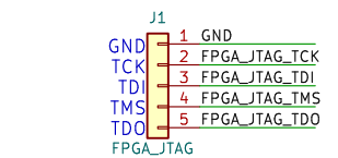
File: ch32h417weu6.kicad_sch
