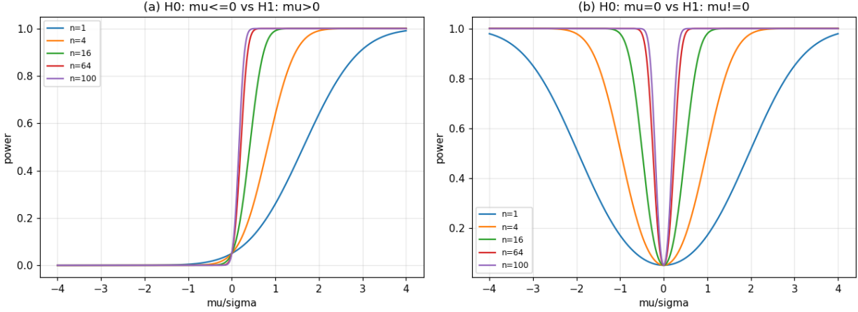
Figure 3: Power functions for 8.12
