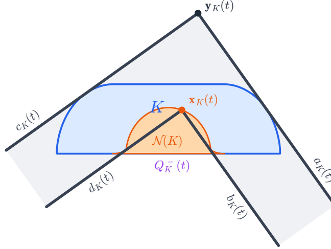
FIGURE 2. A cap, its niche and a supporting hallway: Gerver's cap K = K_G (blue), its niche N(K) (orange), and the supporting hallway L_K(t) at t = 0.62 (grey). The outer walls a_K(t) and c_K(t) of the hallway touch K and meet at the outer corner y_K(t) ; its inner walls b_K(t) and d_K(t) meet at the inner corner x_K(t) , on the boundary of the niche. Q_K^-(t) is the open quarter-plane below the inner corner; the niche is the union of these quarter-planes over t \in (0, \pi/2) , cut at the x -axis.
