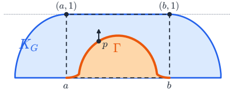
FIGURE 9. Proposition 9.3. Gerver's cap K_G with its niche (orange) below the curve \Gamma formed by \mathbf{D} , \mathbf{x} and \mathbf{B} ; the dashed rectangle [a, b] \times [0, 1] lies in K_G , and \Gamma stays below height one (Fact 2.18). Every point p of \Gamma is a limit of points of G above it.
