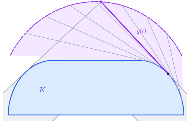
FIGURE 14. One of the terms of \mathcal{Q} in step (4), for Gerber's cap K . For an angle t , the segment of length \varrho(t) runs along an outer wall of the copy of the hallway at the angle t , from the point where K touches that wall (black dot) to the outer corner of the copy (purple dot); the copy at the angle t is drawn in light grey, with its two outer walls touching K . The thin grey segments are the same segment for other angles. As t runs from \varphi to \pi/2 - \varphi , where \varphi = 0.039\dots is Gerber's angle (Appendix B) and this is the range of angles in which the inner corner of the hallway touches Gerber's sofa, the segment sweeps the shaded region, whose area is \frac{1}{2} \int \varrho(t)^2 dt by Mamikon's theorem; the dashed curve is the path of the outer corner.
