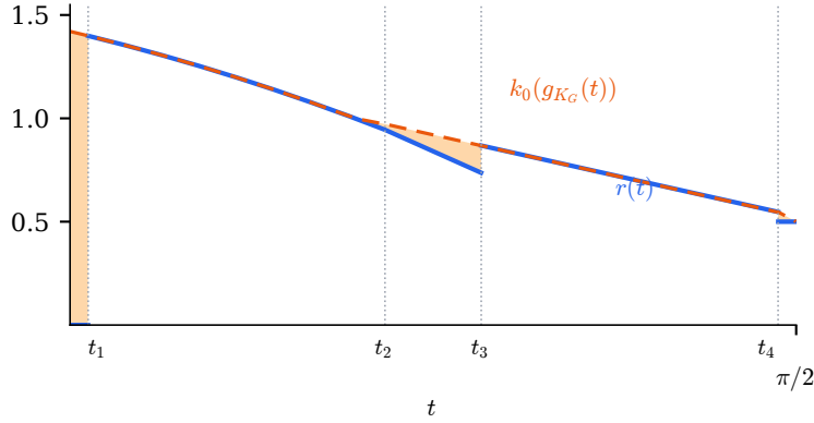
FIGURE 7. The first curvature bound for Gerver's cap, which maximizes \mathcal{A} , as \mathcal{A}(K_G) = |G| (Fact 2.16(b), Fact 2.4(c), Fact 2.7). The density r(t) of \sigma_{K_G} on [0, \pi/2) (blue) and k_0(g_{K_G}(t)) (orange, dashed) are computed from Romik's rotation path. In the figure the blue curve lies below the orange one, and the two agree on [t_1, t_*] and on [t_3, t_4] , where t_* = 0.616\dots is the angle at which g_{K_G} equals 2; the gap between them is shaded.
