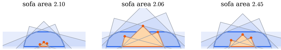
FIGURE 11. Three placements of copies of the hallway at the same three angles t = \pi/8, \pi/4, 5\pi/12 (orange dots: their inner corners). Each copy shades in light blue the region inside its two outer walls, and so do the start and end positions, which keep the sofa in the strip 0 \leq y \leq 1 ; the polygonal cap, outlined in blue, is the darkest region, where all of them overlap, and the polygonal niche (orange) is the part of the cap beyond both inner walls of at least one copy. Left: copies close in give a small cap. Middle: copies far out give a large cap, but also a large niche. Right: a maximum polygon cap for these angles.
