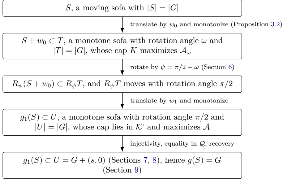
FIGURE 3. The containment chain of the proof. Every set contains the image of S under the maps so far, and all the sets have area |G| ; the first three arrows are a translation followed by a monotoneization, a rotation, and a translation followed by a monotoneization. Here g_1(p) = R_\psi(p + w_0) + w_1 and g(p) = g_1(p) - (s, 0) .
