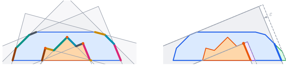
FIGURE 12. Balance of the maximum polygon cap of Figure 11. Left: the three copies of the hallway (light grey; orange dots: their inner corners); each slanted side of the cap lies on an outer wall of one of the copies, and is drawn thick in the same colour as the side of the niche on the inner wall of the same copy parallel to it; the two have the same length. A side of the niche may consist of several pieces, as for the amber pair. Right: Gerver's balancing argument. The copy at the angle \pi/8 (light grey) is moved outward by \varepsilon (dashed), which moves one of its outer walls and the inner wall parallel to it and leaves the other two walls in place. This adds to the cap a strip along its side on that wall (green), and to the niche a strip along its side on the inner wall (purple); the two sides are drawn thick. The sofa area changes by about \varepsilon times the difference of their lengths, so if they differed, moving the walls outward or inward would increase it; here the two sides have the same length, 0.63, as they do at each of the six slanted sides of this cap.
