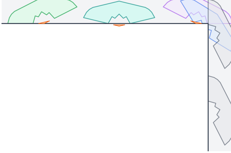
FIGURE 13. Step (3a) for an actual sofa: a polygonal cap with rotation angle \omega = 1.1 (about 63^\circ ) minus its niche. A copy of the sofa turned by \pi/2 - \omega (green) first turns back inside the horizontal side, before the corner, through the position halfway (teal), to the sofa's own starting position (purple). This is possible because the small triangle at the inner corner (orange) lies in the hollow of the sofa, which keeps its height at most 1 throughout this turn. The copy then follows the sofa's own movement and turns by \omega around the corner (blue halfway, grey at the end, and again slid down the vertical side). In total, it turns by the full right angle.
