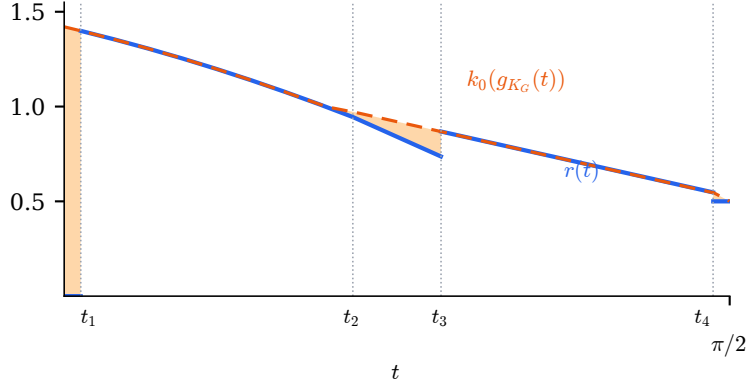
FIGURE 7. The first curvature bound for Gerver's cap, which maximizes \mathcal{A} , as \mathcal{A}(K_G) = |G| (Fact 2.35(b), Fact 2.11(c), Fact 2.15). The density r(t) of \sigma_{K_G} on [0, \pi/2) (blue) and k_0(g_{K_G}(t)) (orange, dashed) are computed from Romik's rotation path. In the figure the blue curve lies below the orange one, and the two agree on [t_1, t_*] and on [t_3, t_4] , where t_* = 0.616\dots is the angle at which g_{K_G} equals 2; the gap between them is shaded.
