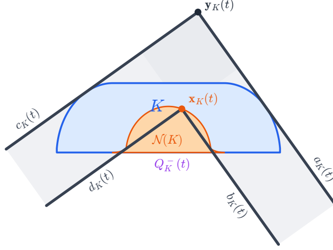
FIGURE 2. A cap, its niche and a supporting hallway: Gerver's cap K = K_G (blue), its niche \mathcal{N}(K) (orange), and the supporting hallway L_K(t) at t = 0.62 (grey), whose outer walls a_K(t) and c_K(t) touch K and meet at the outer corner \mathbf{y}_K(t) , and whose inner walls b_K(t) and d_K(t) meet at the inner corner \mathbf{x}_K(t) , on the boundary of the niche. Q_K^-(t) is the open quarter-plane below the inner corner; the niche is the union of these quarter-planes over t \in (0, \pi/2) , cut at the x -axis.
