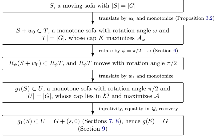
FIGURE 3. The containment chain of the proof. Every set contains the image of S under the maps so far, and all the sets have area |G| ; the first three arrows are a translation followed by a monotone, a rotation, and a translation followed by a monotone. Here g_1(p) = R_\psi(p + w_0) + w_1 and g(p) = g_1(p) - (s, 0) .
