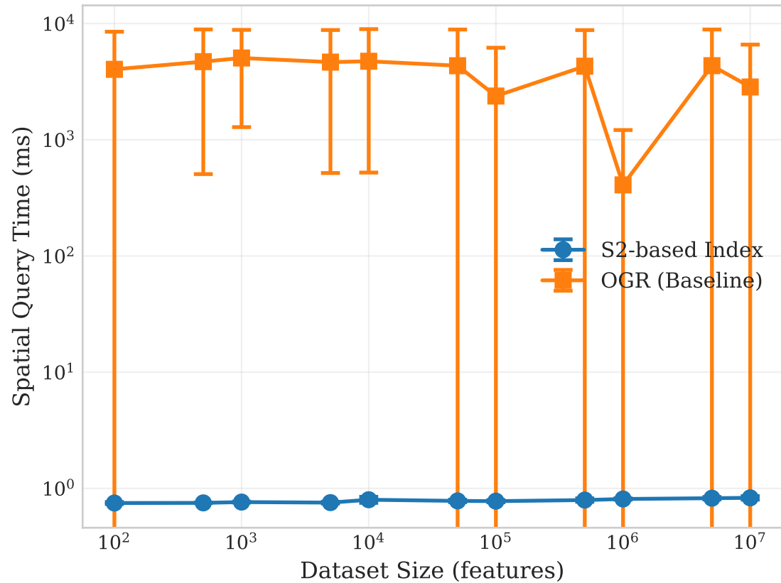
(a) Spatial Query Performance
