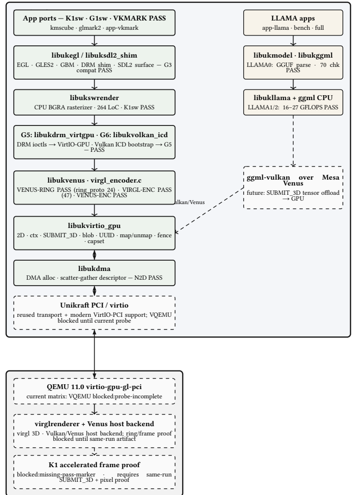
Figure 1: VOGUE software stack (current state).
