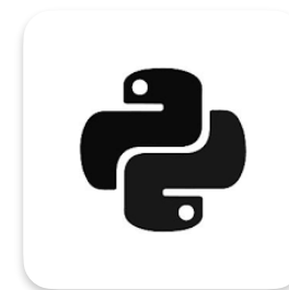
build_ppe_json.py
