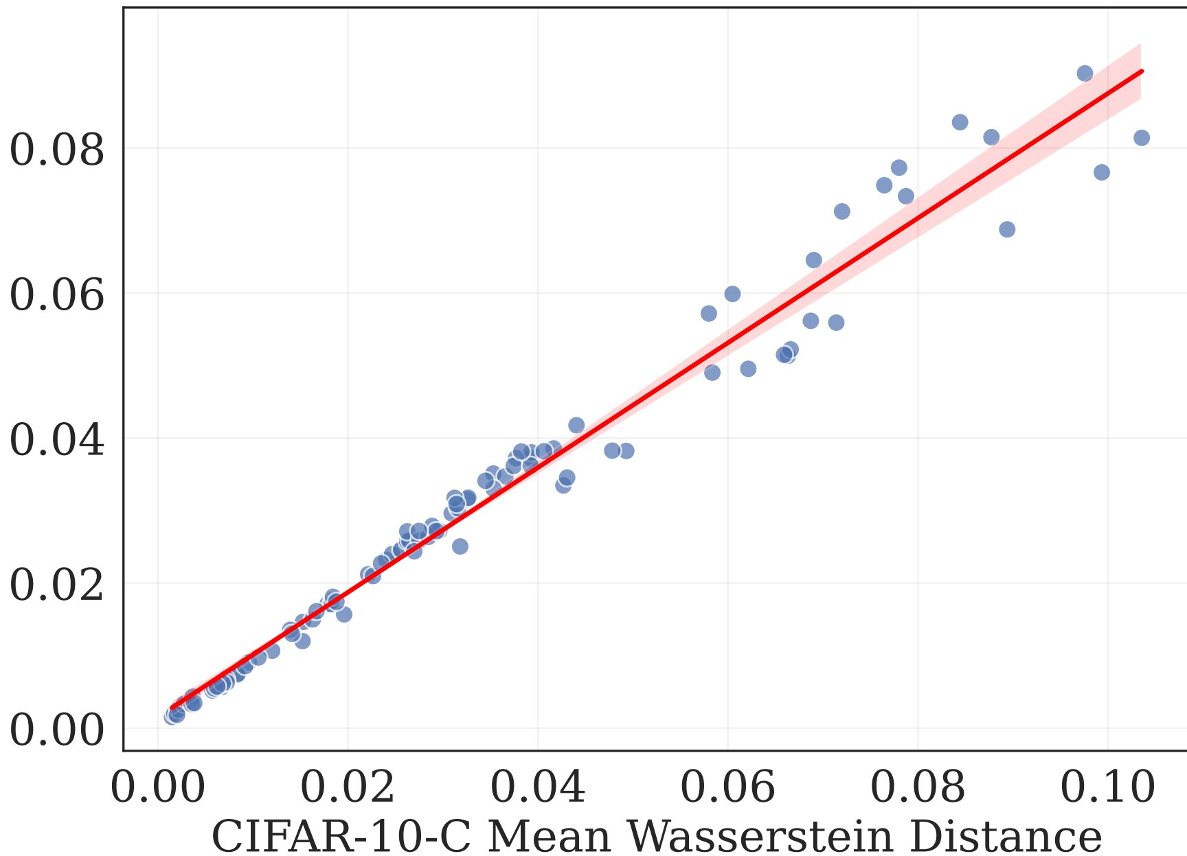
CIFAR-10-C vs CIFAR-100-C Correlation Pearson r=0.987 , Spearman r=0.994
