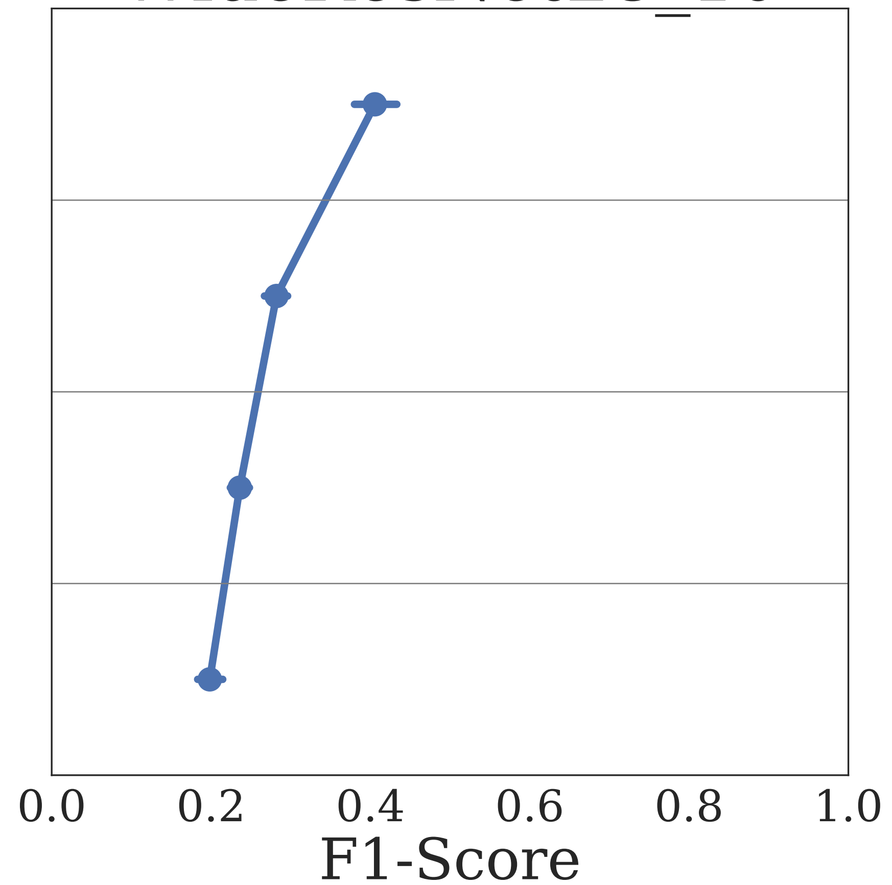
WideResNet28_10
