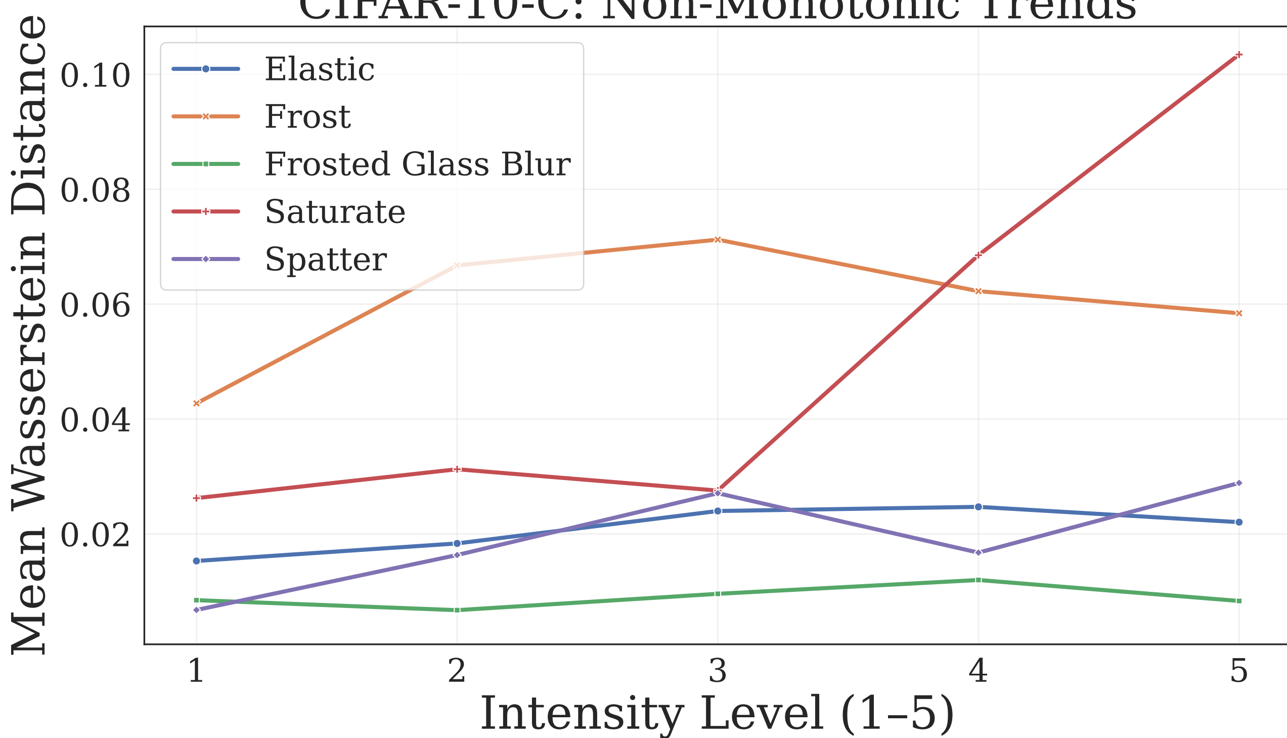
CIFAR-10-C: Non-Monotonic Trends
