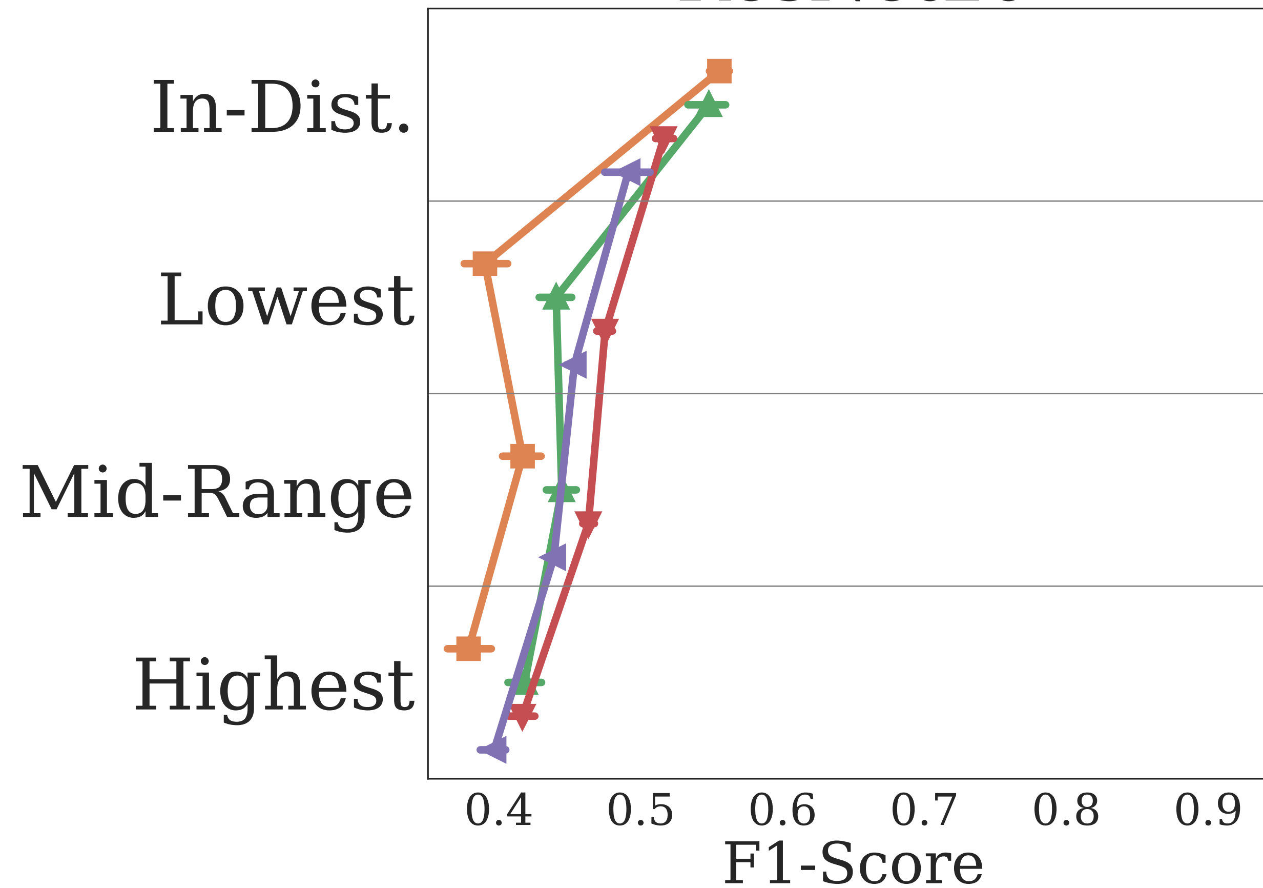
ResNet20
