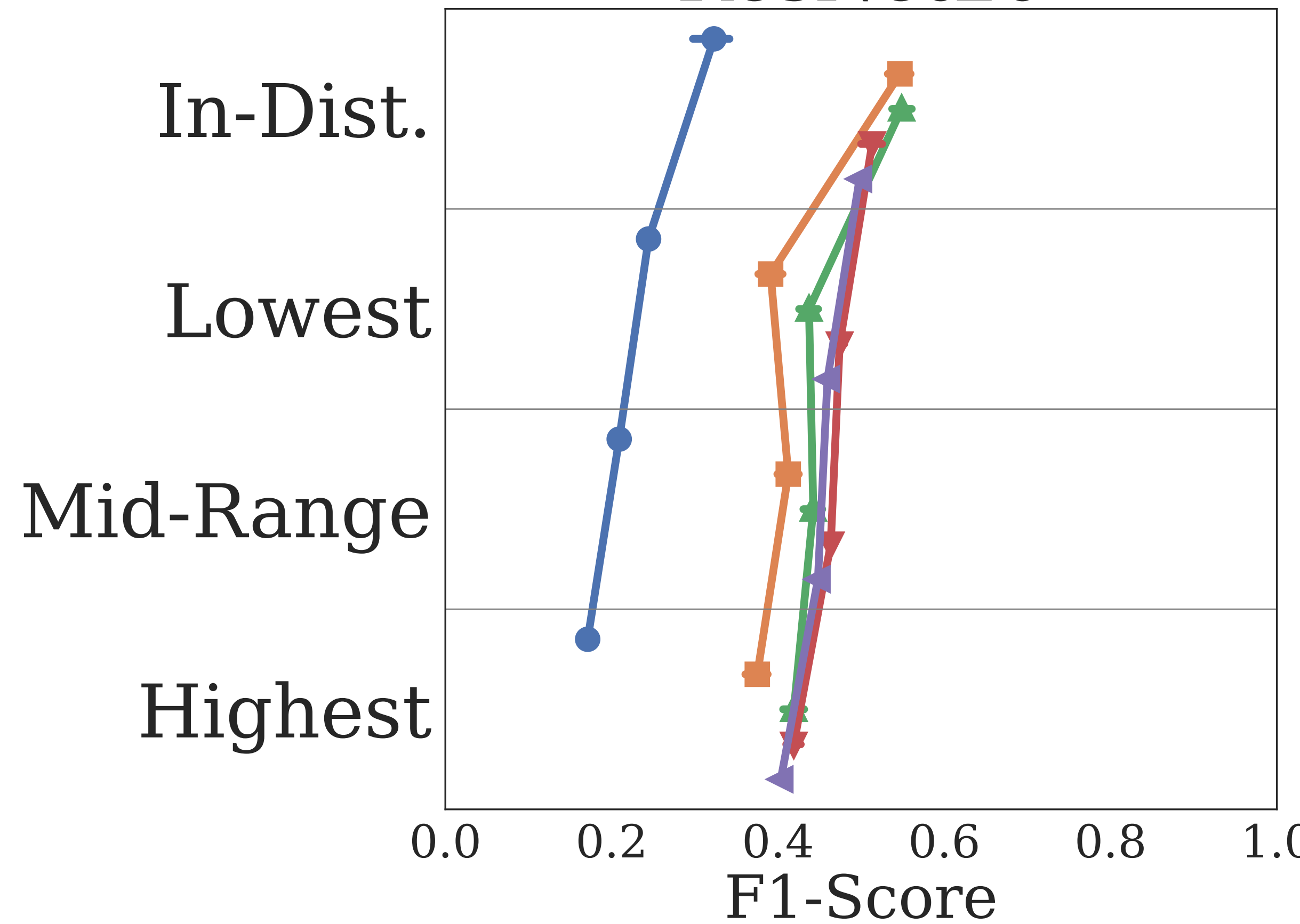
ResNet20
