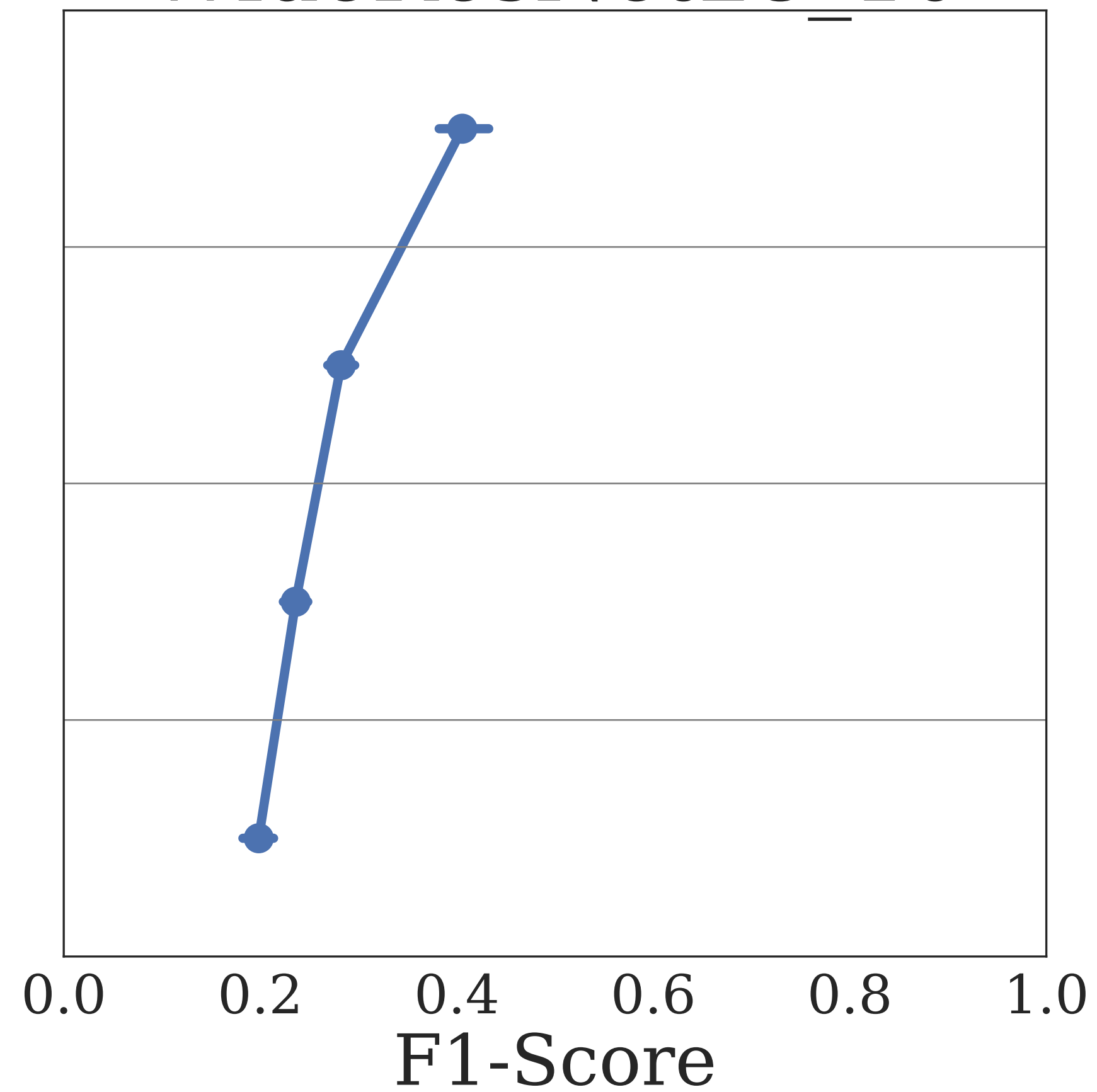
WideResNet28_10
