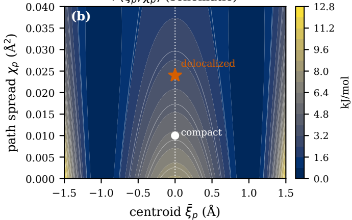
F(\bar{\xi}_p, \chi_p) (schematic)
