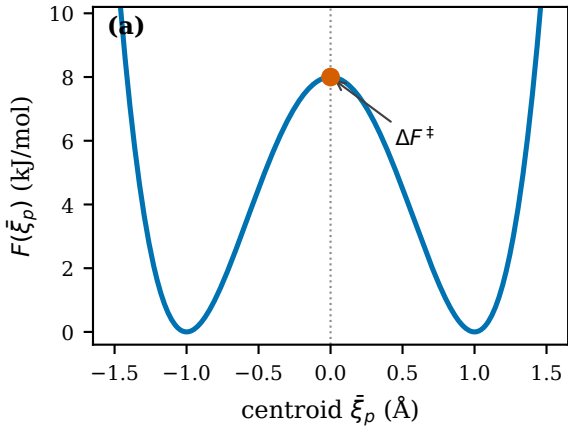
Centroid PMF (schematic)
