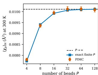
FIG. 3. Bead convergence of \langle \chi_p \rangle_H at 300 K. The primitive PIMC estimator follows the exact finite- P formula, Eq. (8), and both approach the continuum, Eq. (7).
