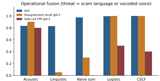
Figure 2: Fusion on operational threat labels. ShieldCall and logistic regression recover disagreement cells that a naive sum misses, and both pay in false positives on safe calls at the 0.5 threshold.
