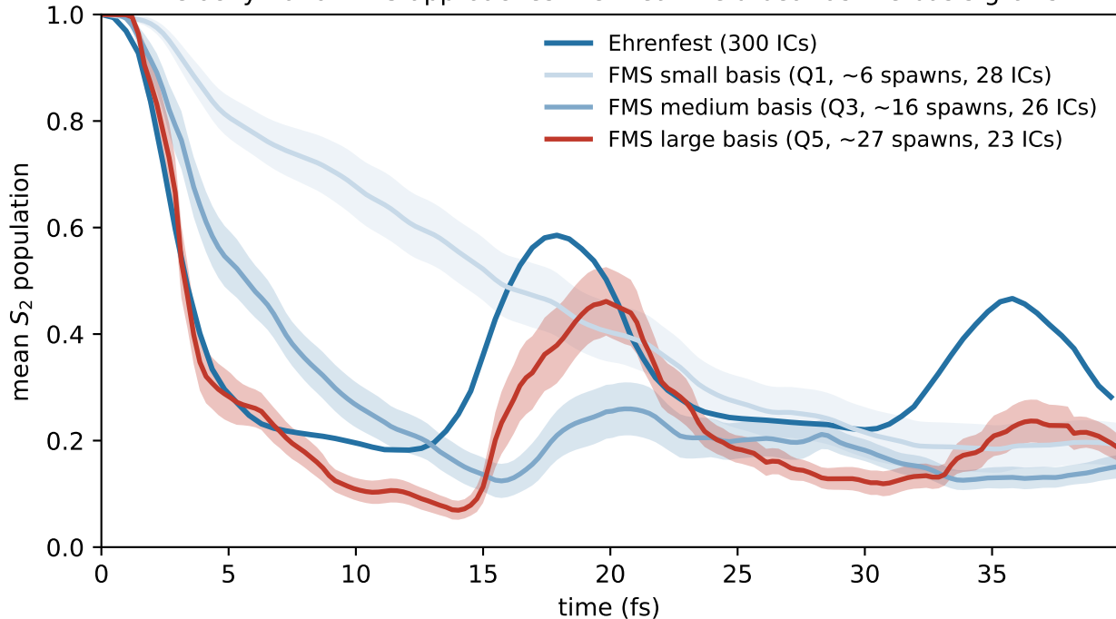
velocity-flavor FMS approaches the mean-field beat as the basis grows
