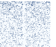
PR WT +ligand RUNX motif
