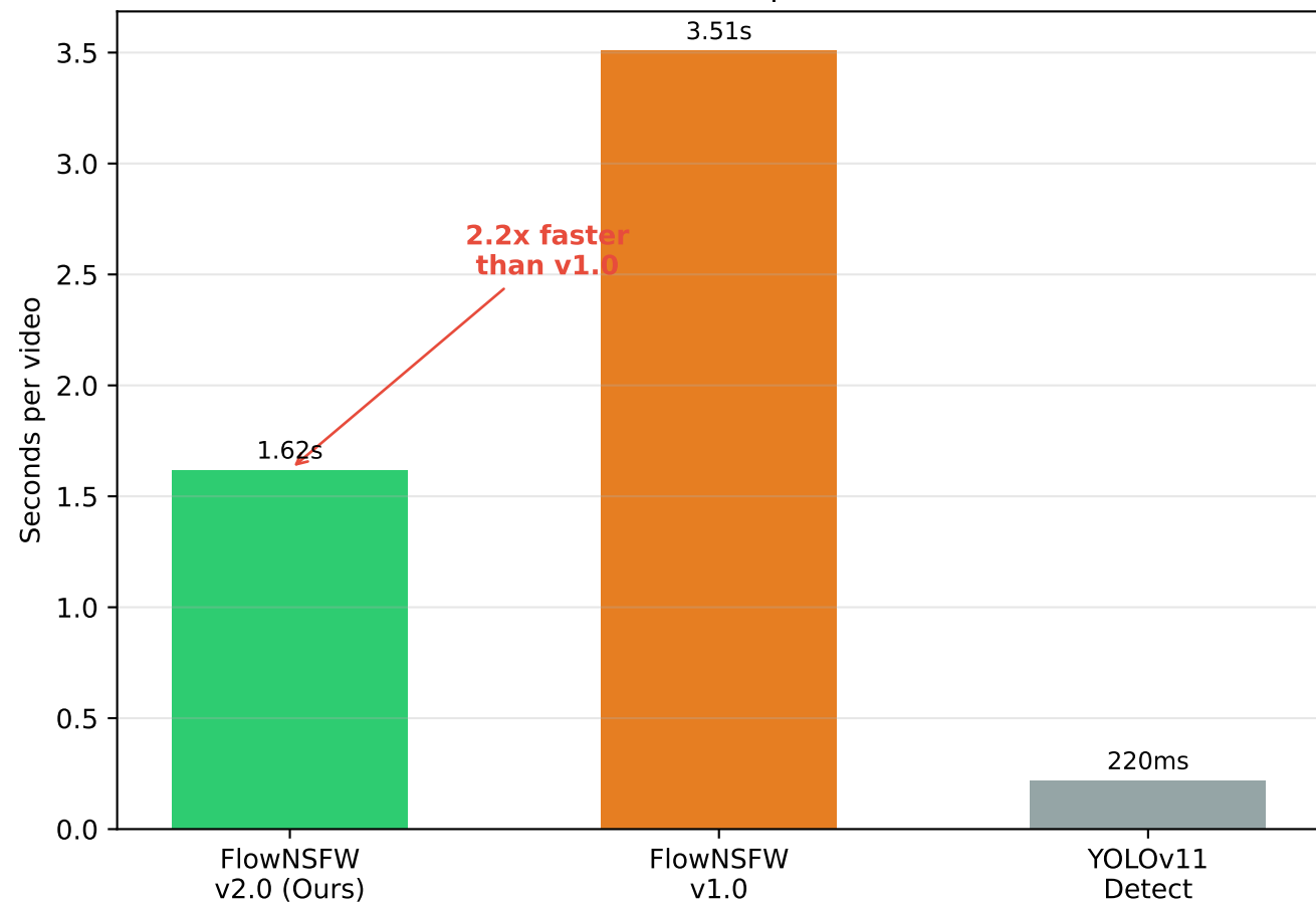
Inference Speed
