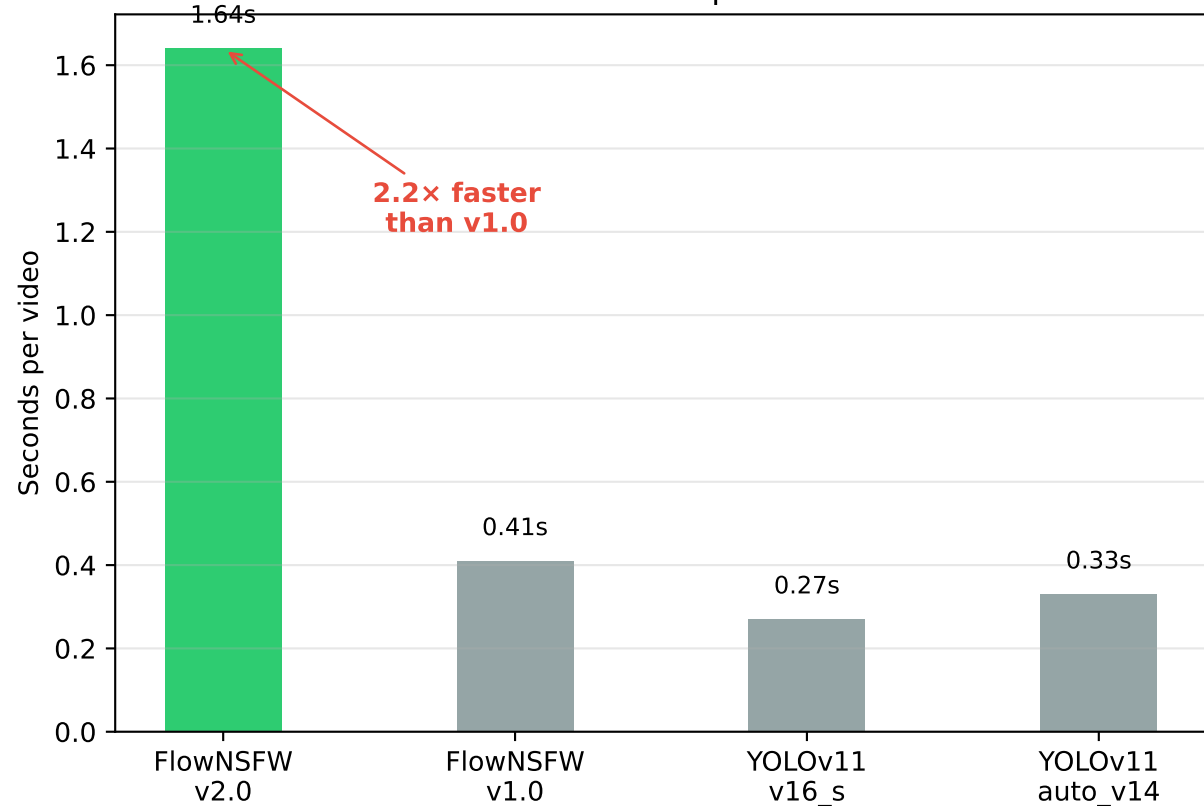
Inference Speed
