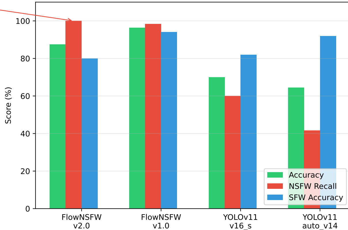
Detection Performance
