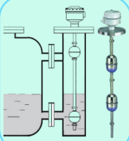
LEVEL SWITCH WITH EXTERNAL CHAMBER
