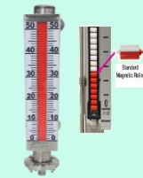
SIDE MOUNTED MAGNETIC LEVEL INDICATOR (BI-COLOUE FLAPPER DESIGN)
