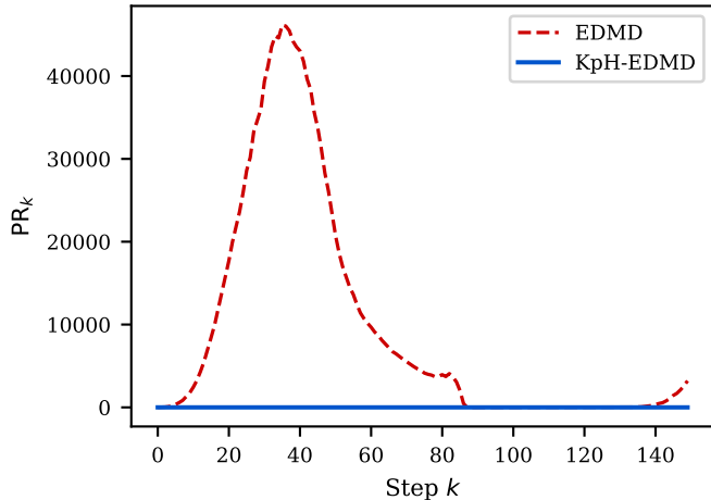
Passivity residual
