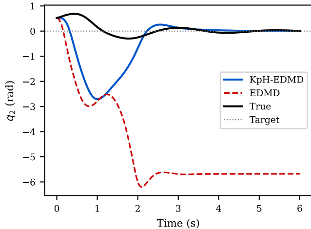
Joint 2
