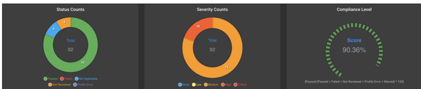
Figure 2: Overall Compliance for Kubernetes
