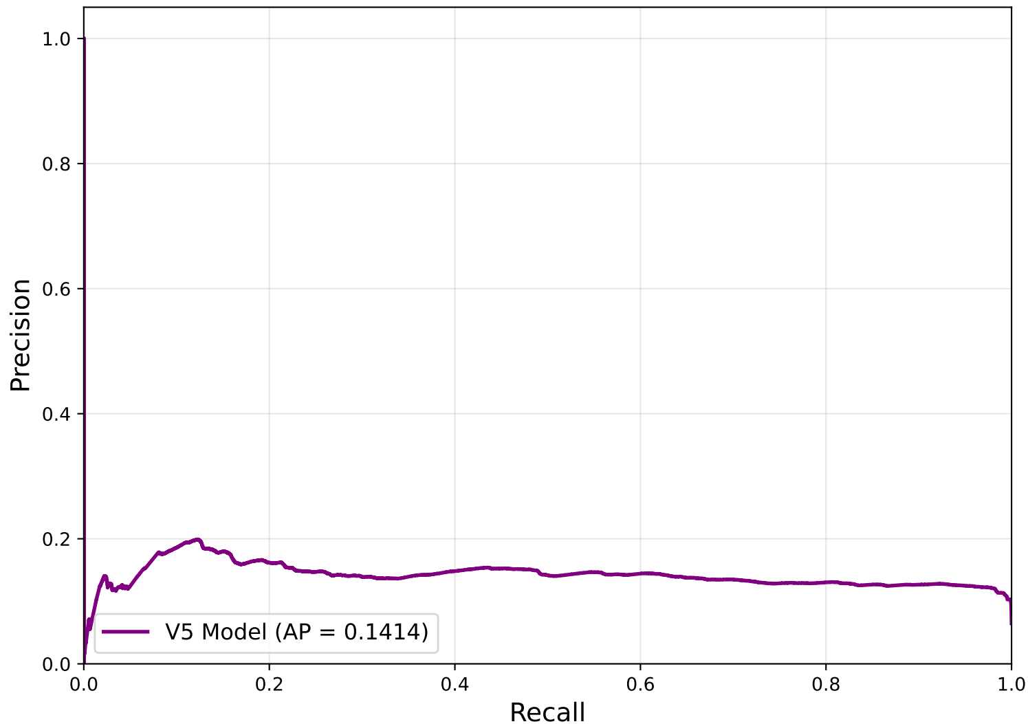
Frame-Level Precision-Recall Curve
