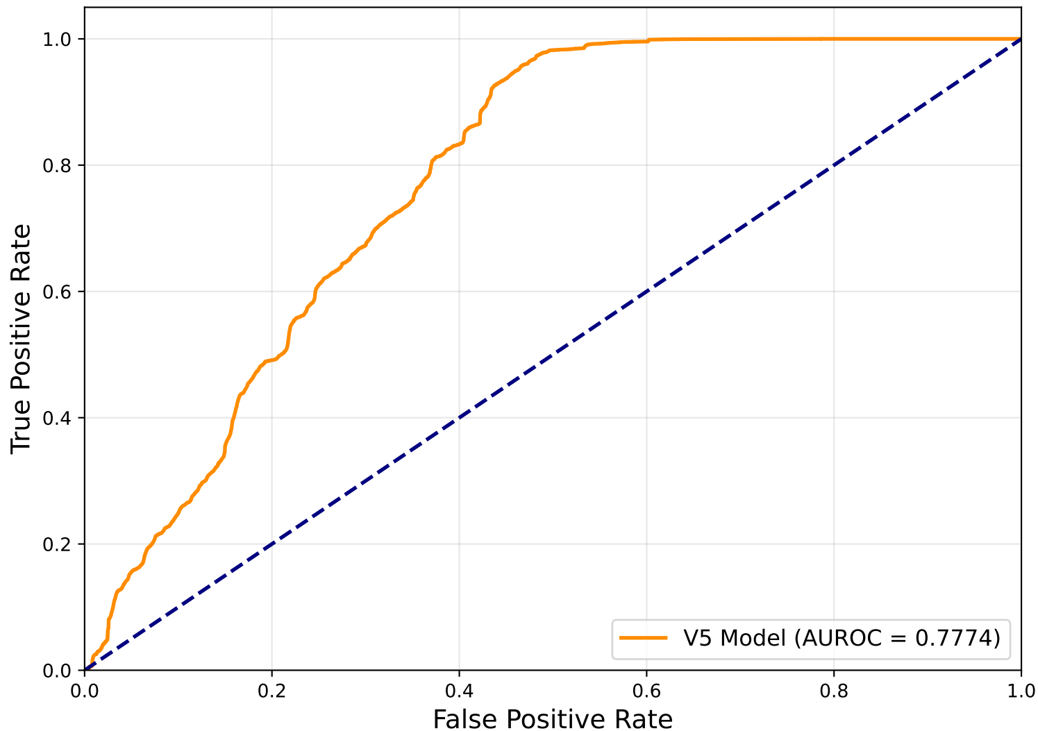
Frame-Level ROC Curve on UCF-Crime
