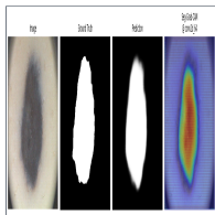
Seg-Grad-CAM
