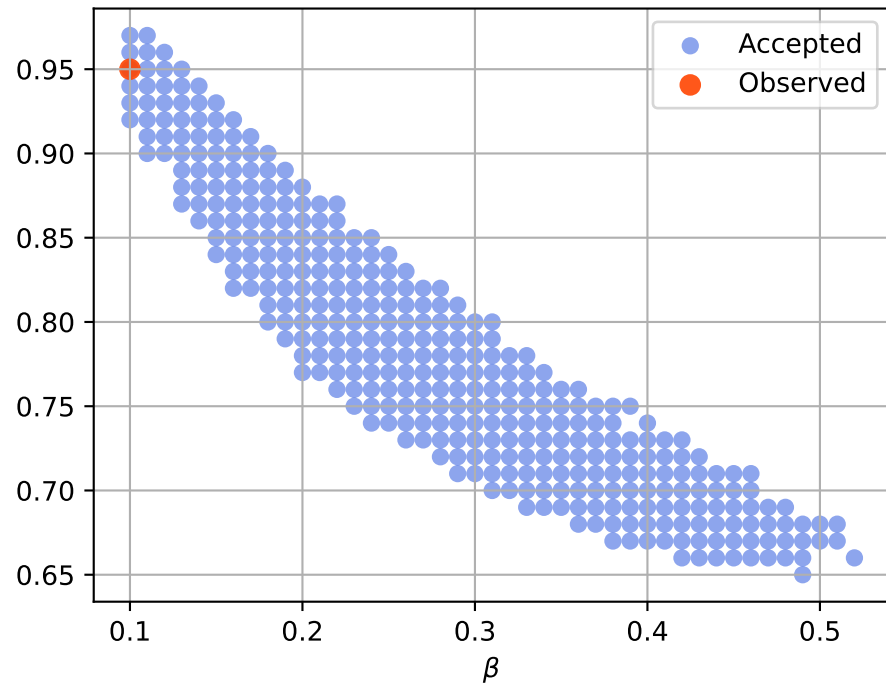
Accepted parameters - History Matching
