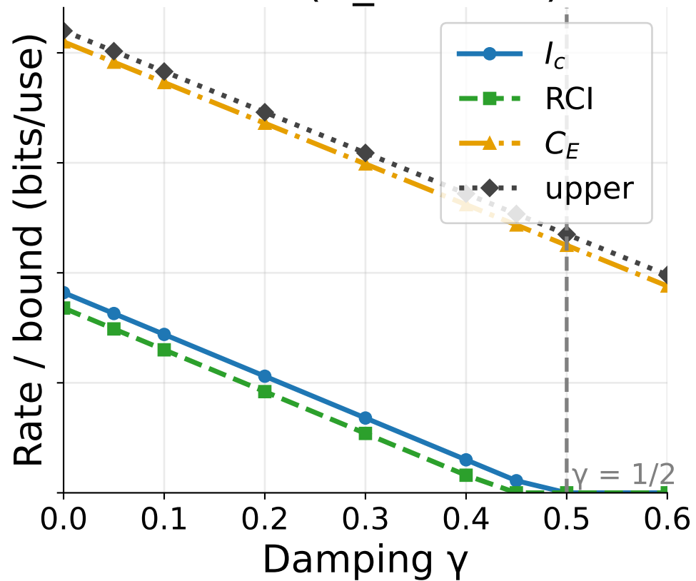
GADC ( N_{th} = 0.1 )
