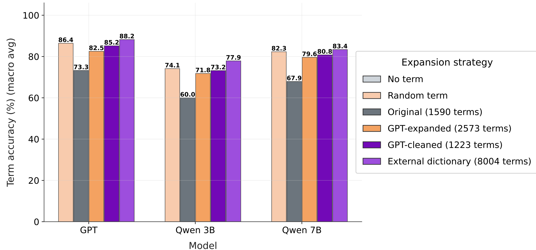
Terminology expansion across models (dev_v1; macro avg over language pairs)
