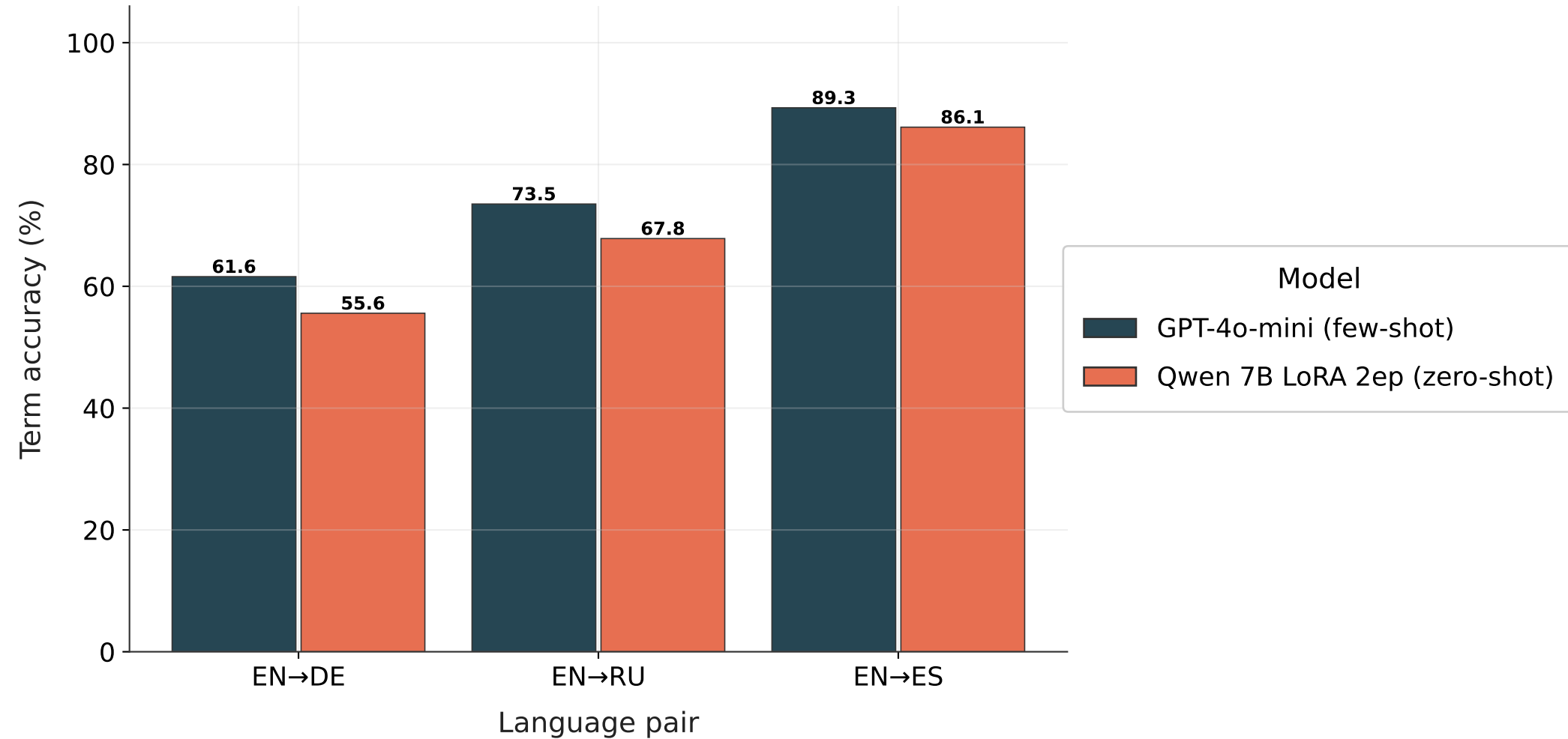
Best LoRA config vs. GPT-4o-mini (train dev_v2; test dev_v1; proper_term)
