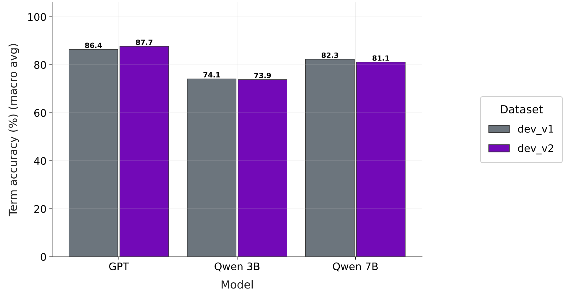
dev_v1 vs dev_v2 terminology datasets (random_term; macro avg over language pairs; per model)
