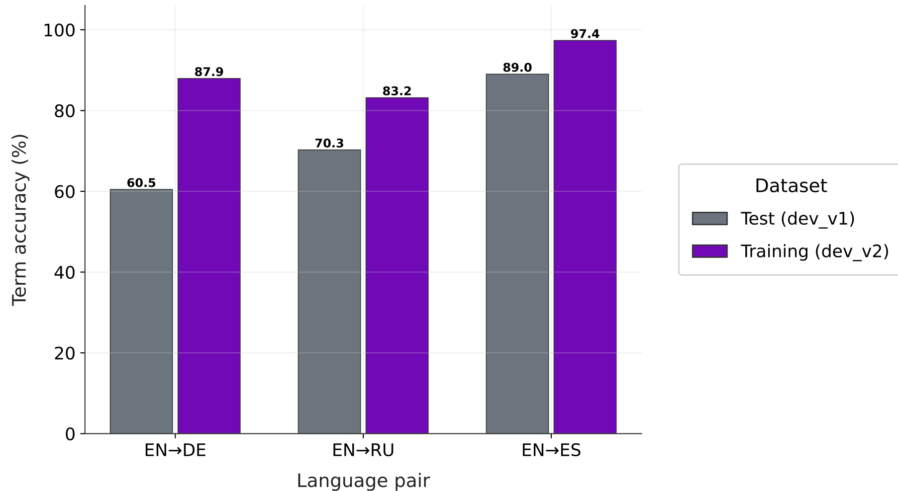
Test vs training terminology datasets (proper_term; GPT-4o-mini; per language pair)
