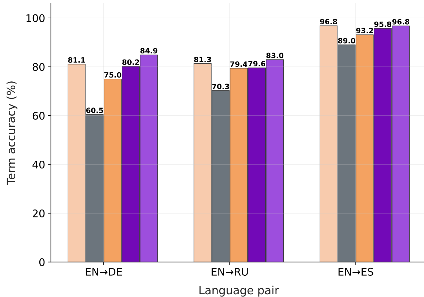
Terminology expansion by language pair (dev_v1; GPT)
